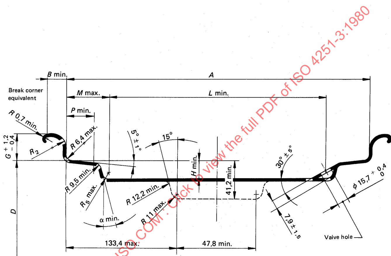
Figure 2 — Contour of W and DW rims
