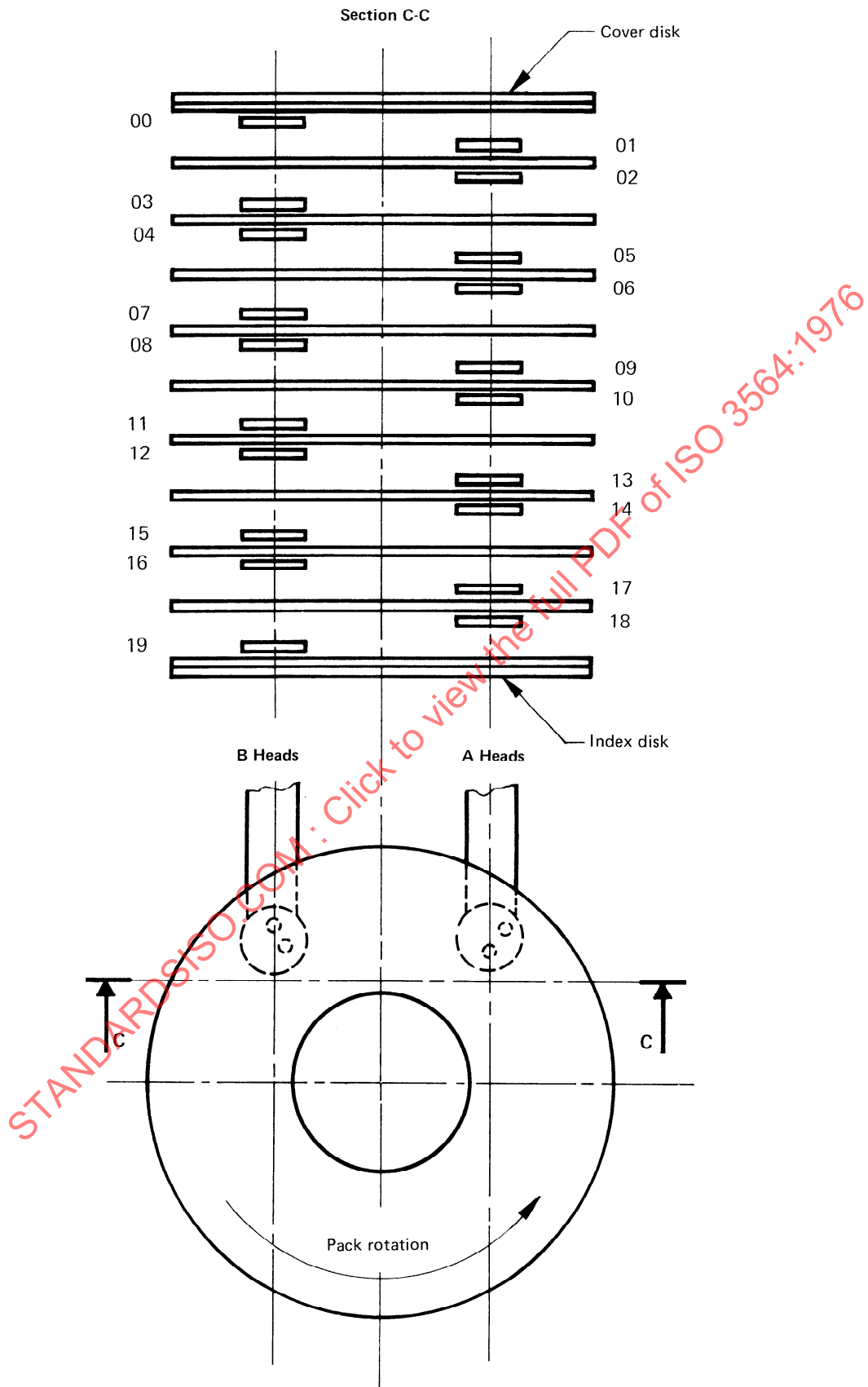
FIGURE 6 — Disk rotation and designations of disk surfaces and heads
