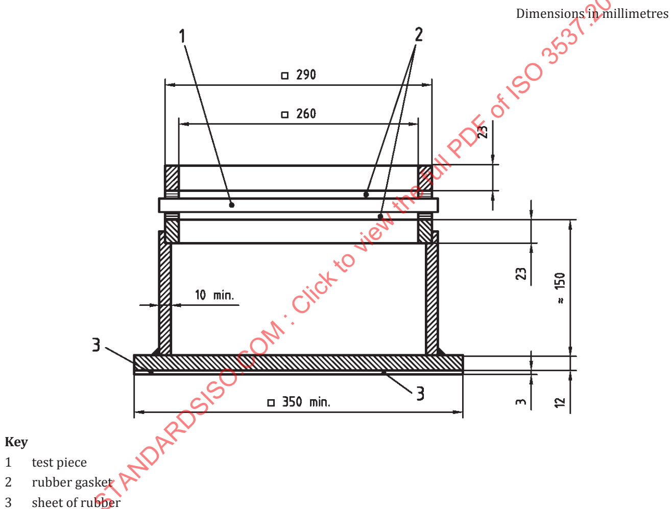
Figure 1 — Support for ball tests
