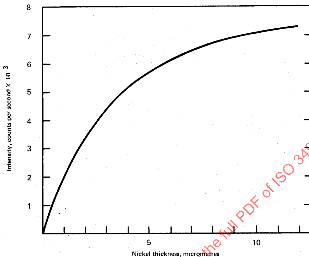
FIGURE 1 — Calibration curve for the determination of a nickel thickness by X-ray emission
