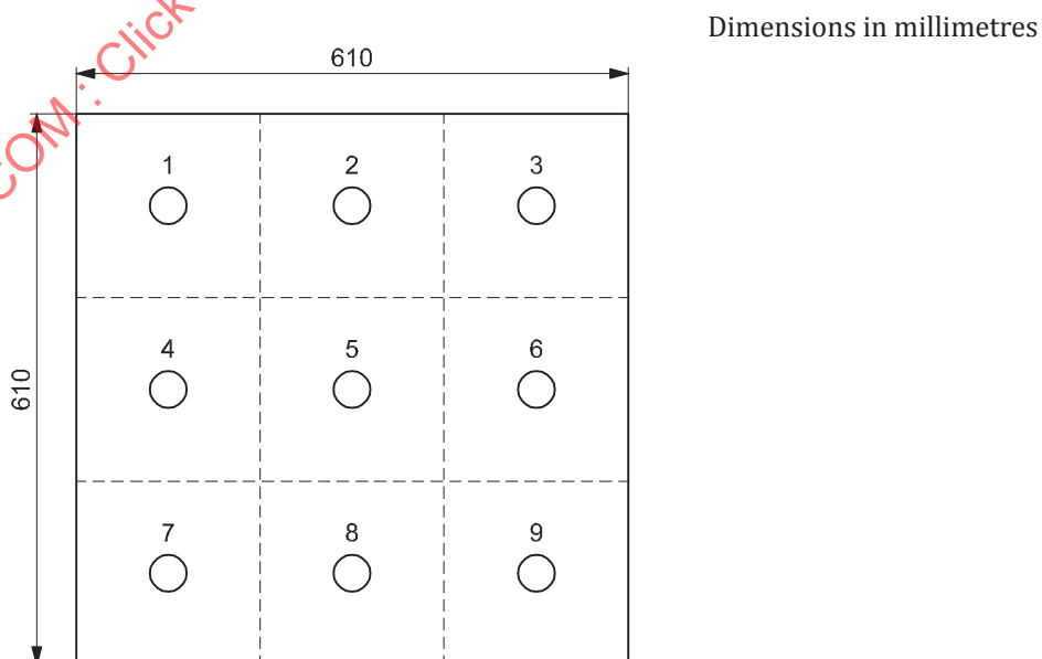
Figure 12 — Air velocity and aerosol uniformity: sampling points for measuring uniformity of air velocity and aerosol dispersion
