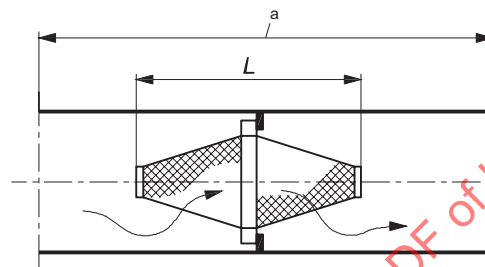
Figure 3 — Dimensions of the test rig
