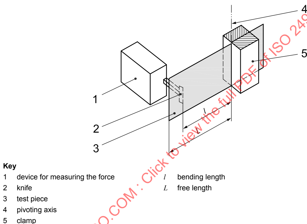
Figure 1 — Sketch of the bending resistance testing
