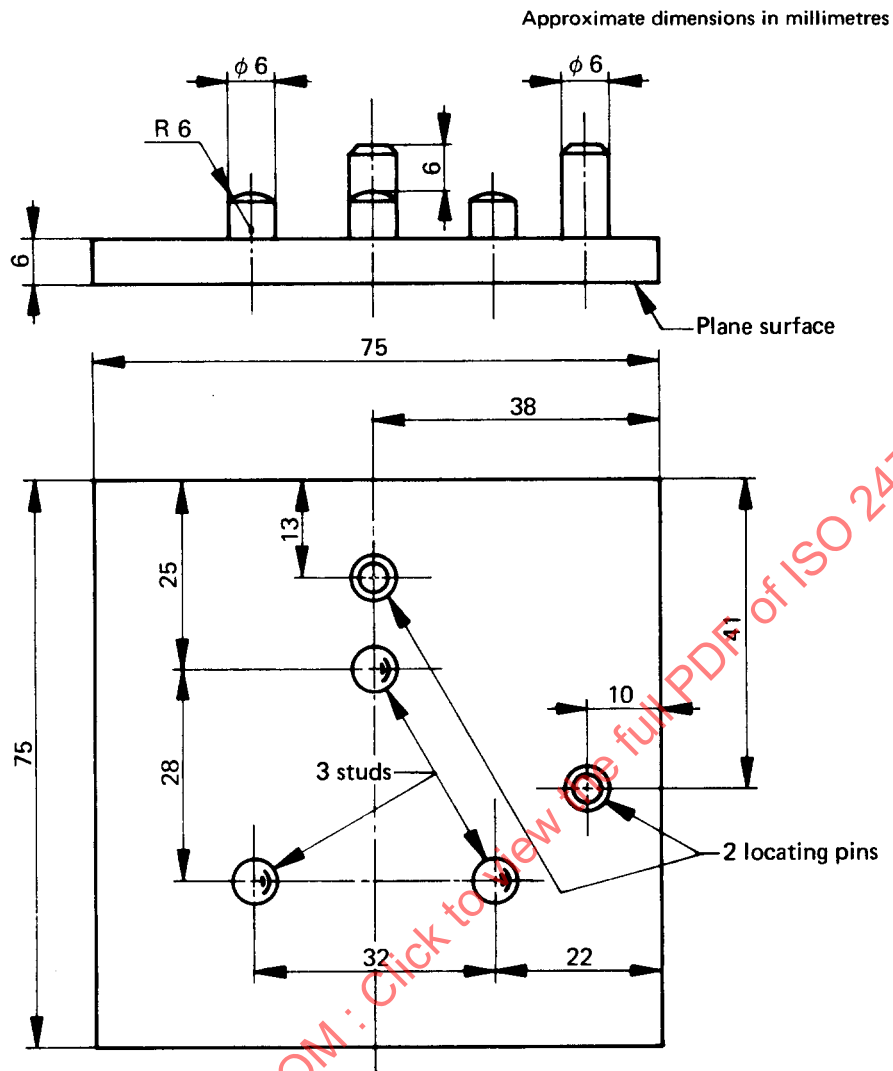
♦ FIGURE 1 – Carrier for the test piece
