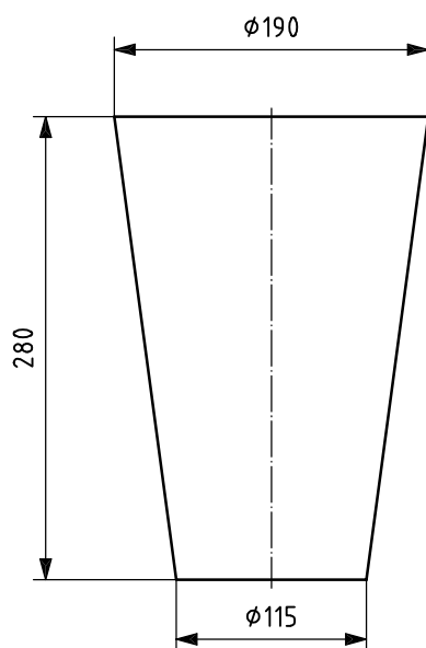
Figure C.3 — Test sample dimensions trans-femoral (above-knee) — Socket former
