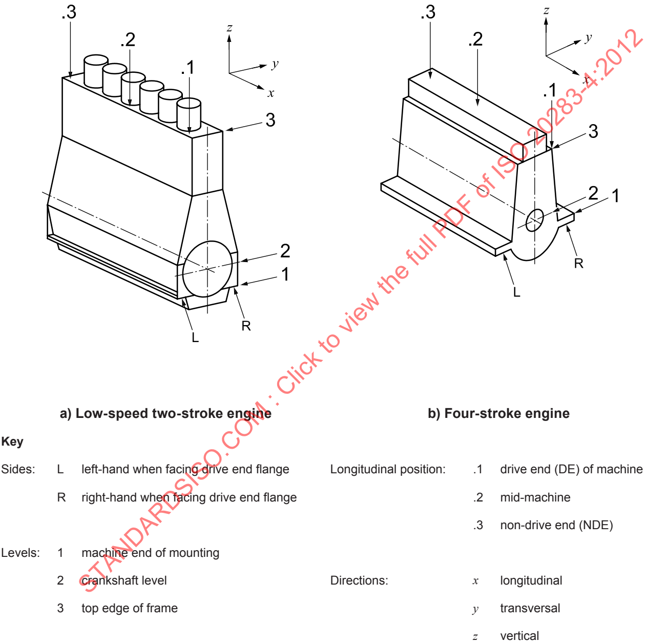
Figure 2 — Typical measurement points on a diesel engine
