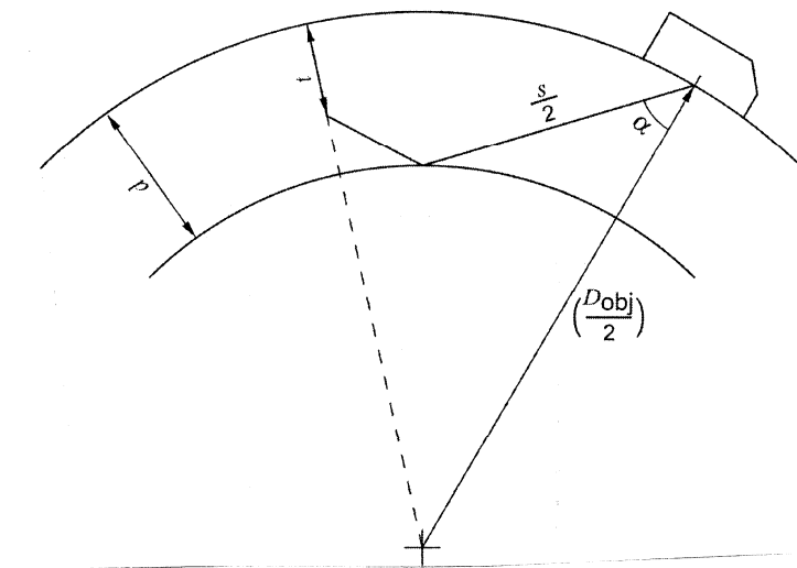
Figure C.2 — Determination of sound path distance for scanning from the outer surface in full skip
