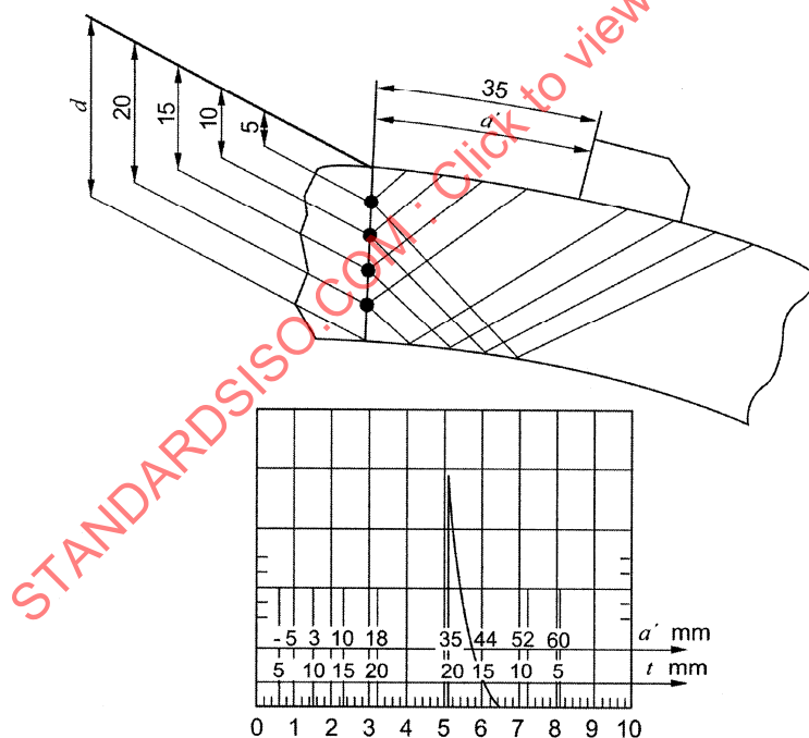
Figure 7 — Definitions for setting of the timebase in terms of e. g. reduced projection distance
