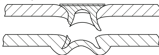
b) Pull out of the rivet head
