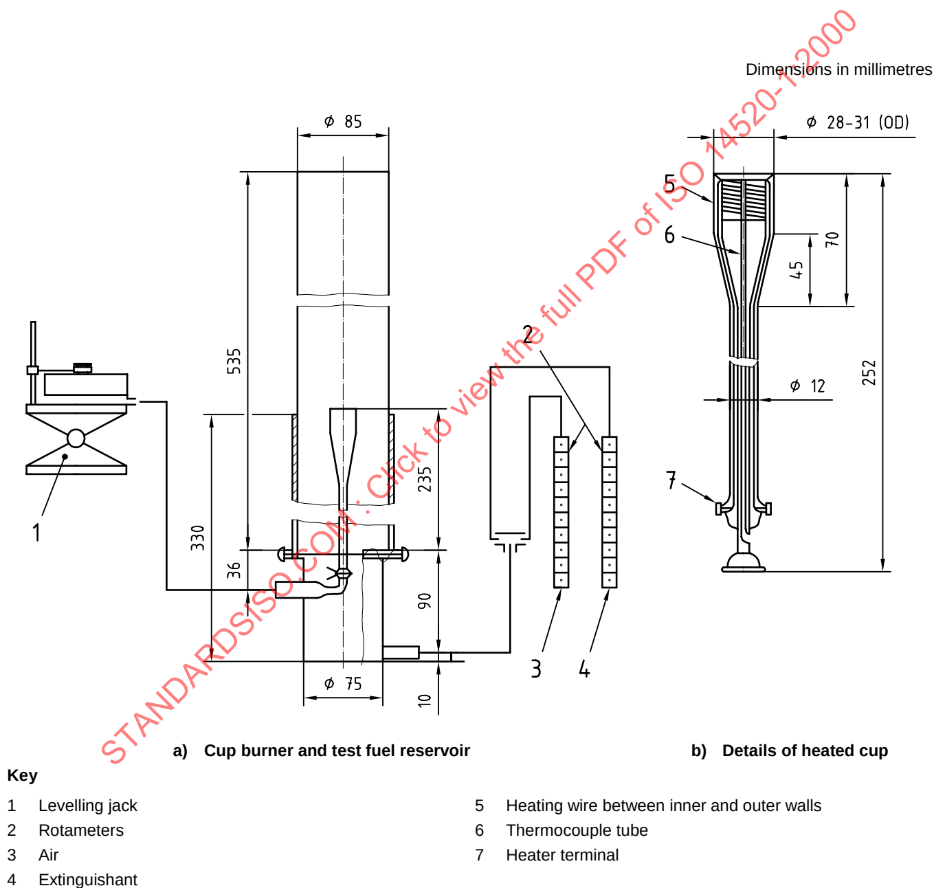
Figure B.1 — Cup burner apparatus
