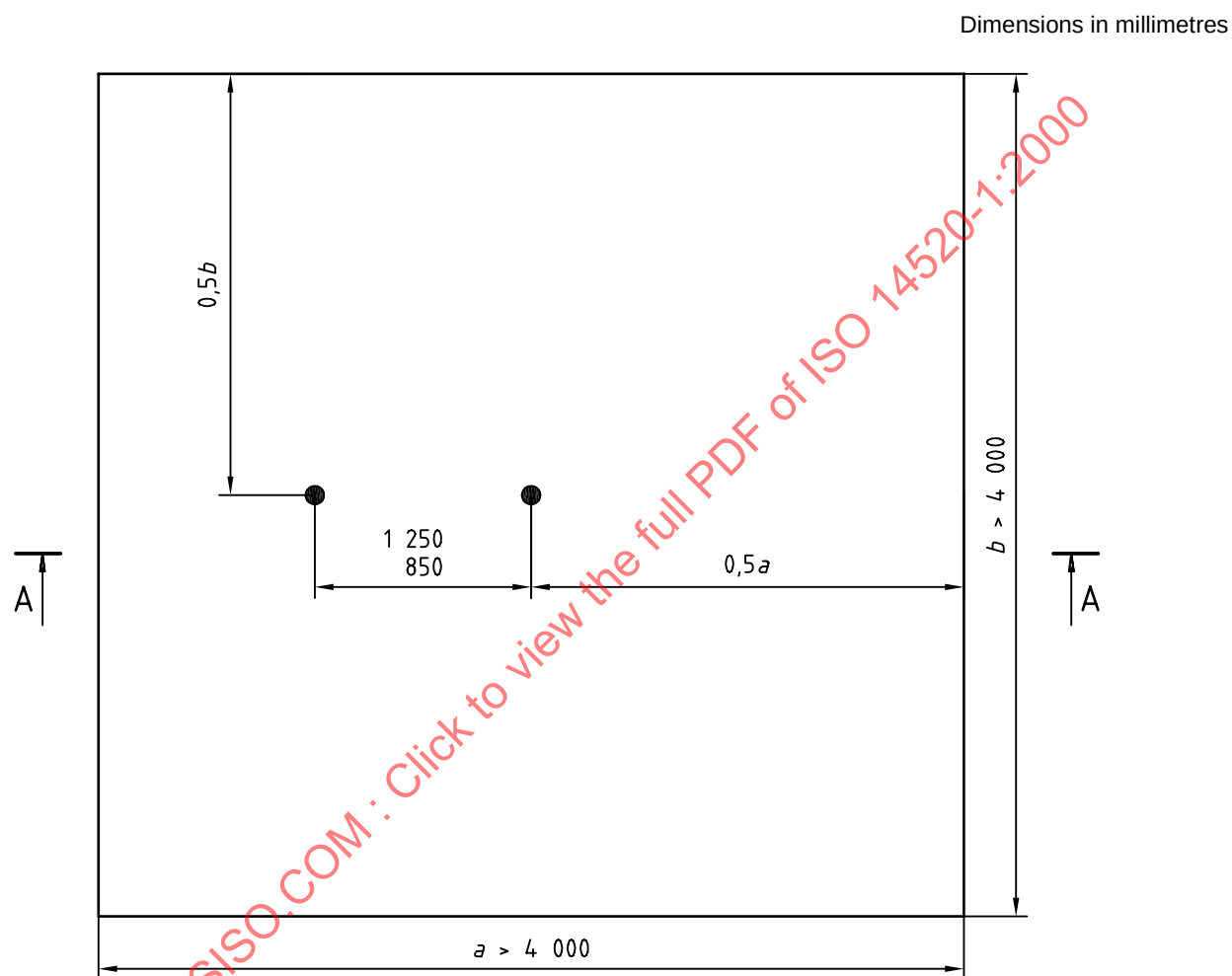
Figure C.2 — Plan view of instrumentation placement for nozzle minimum height/maximum area coverage test
