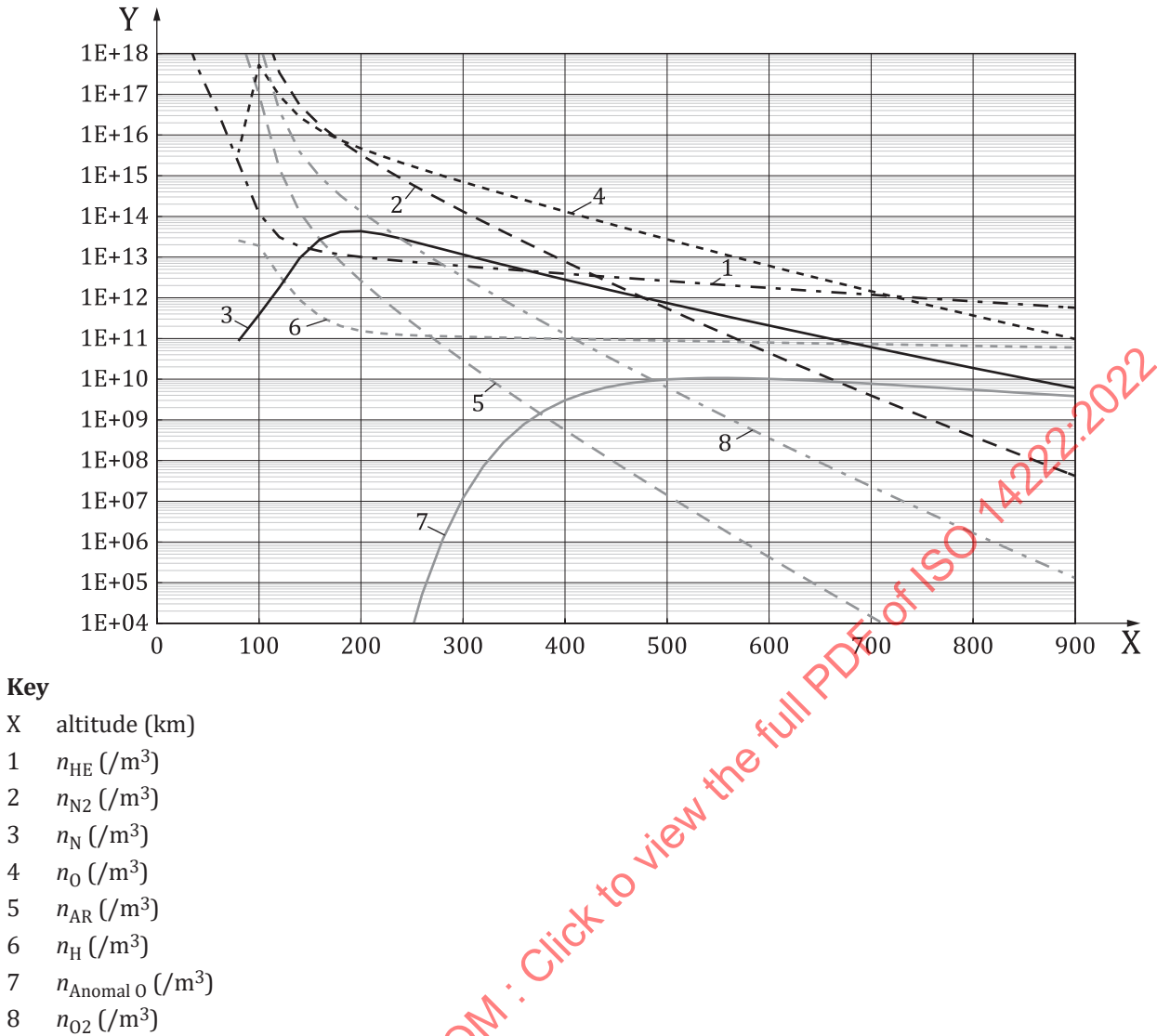
Figure A.3 — NRLMSIS 2.0 mean concentration of atmosphere constituents for moderate solar and geomagnetic activity
