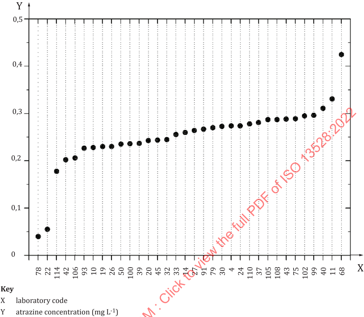
Figure E.1 — Ranked participant results for Atrazine (data from Table E.4 )
