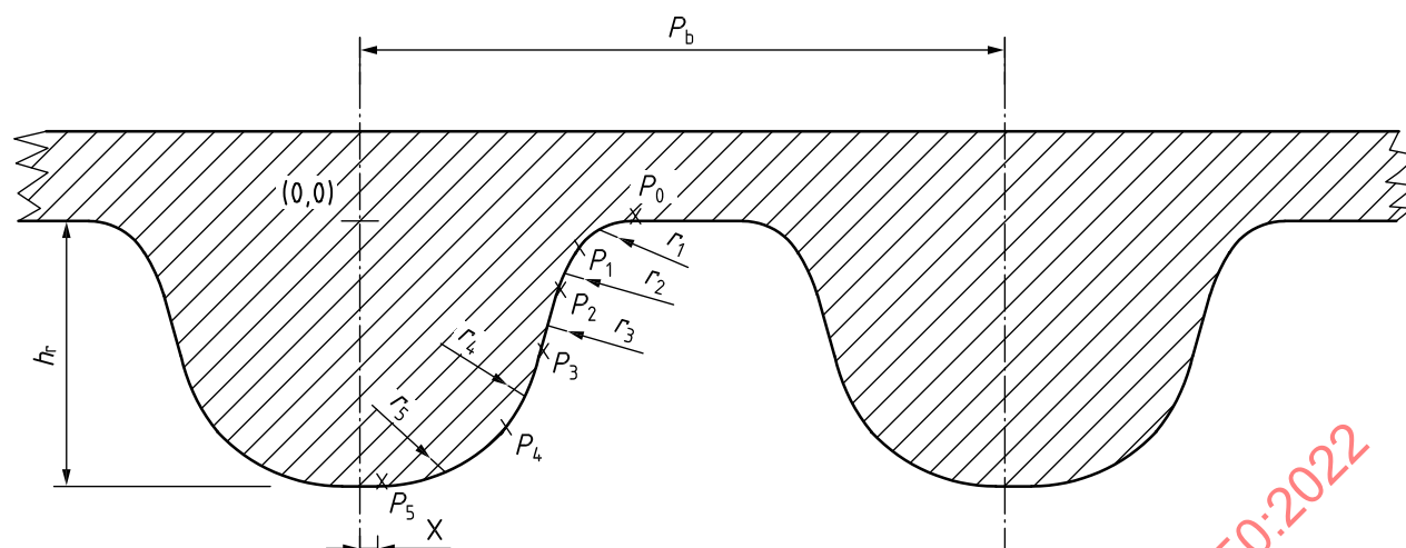
Figure 10 — Pulley generating tool rack form
