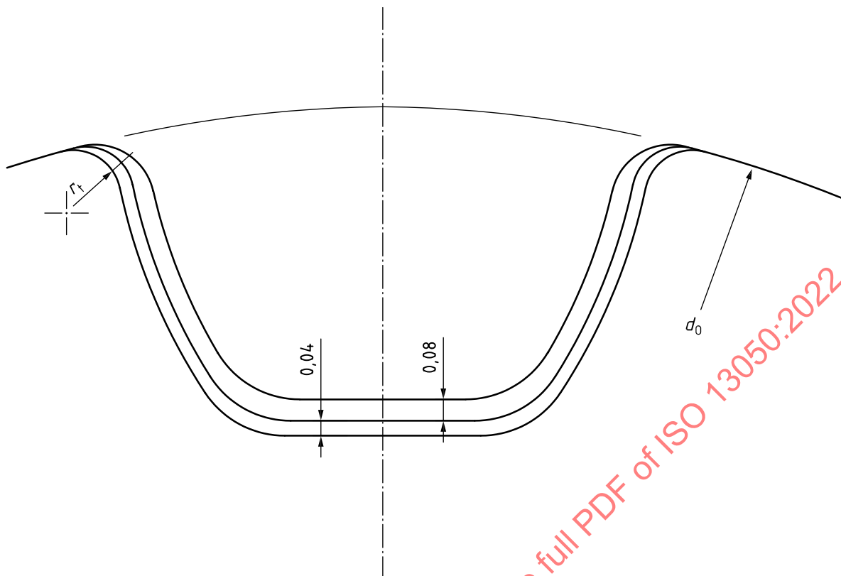
Figure 18 — Pulley groove tolerance band
