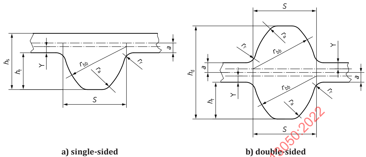
Figure 21 — Tooth dimensions – Profile system S
