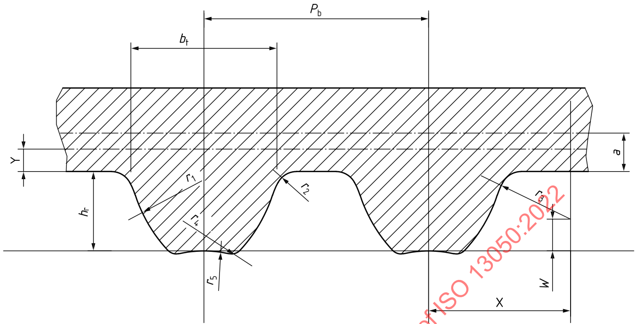
Figure 23 — Pulley generating tool rack form
