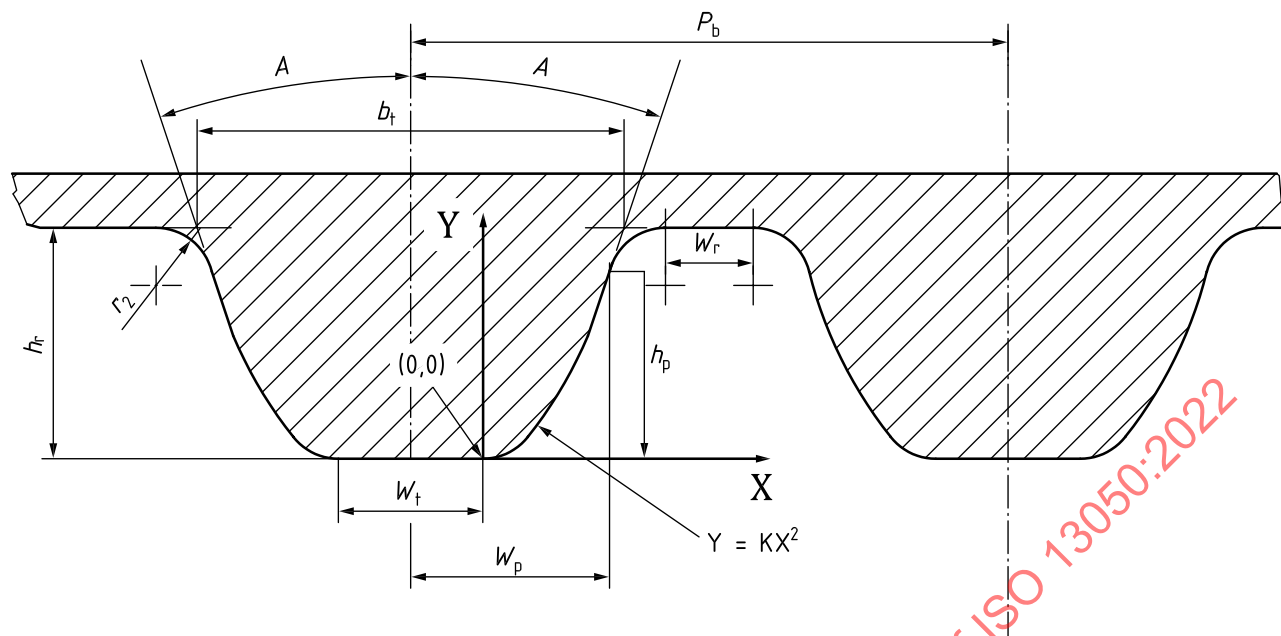
Figure 16 — Pulley generating tool rack form
