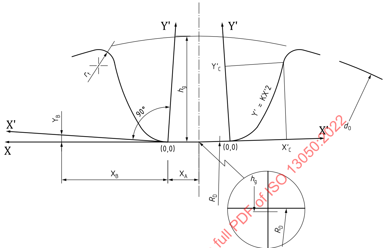
Figure 17 — Pulley groove profile
