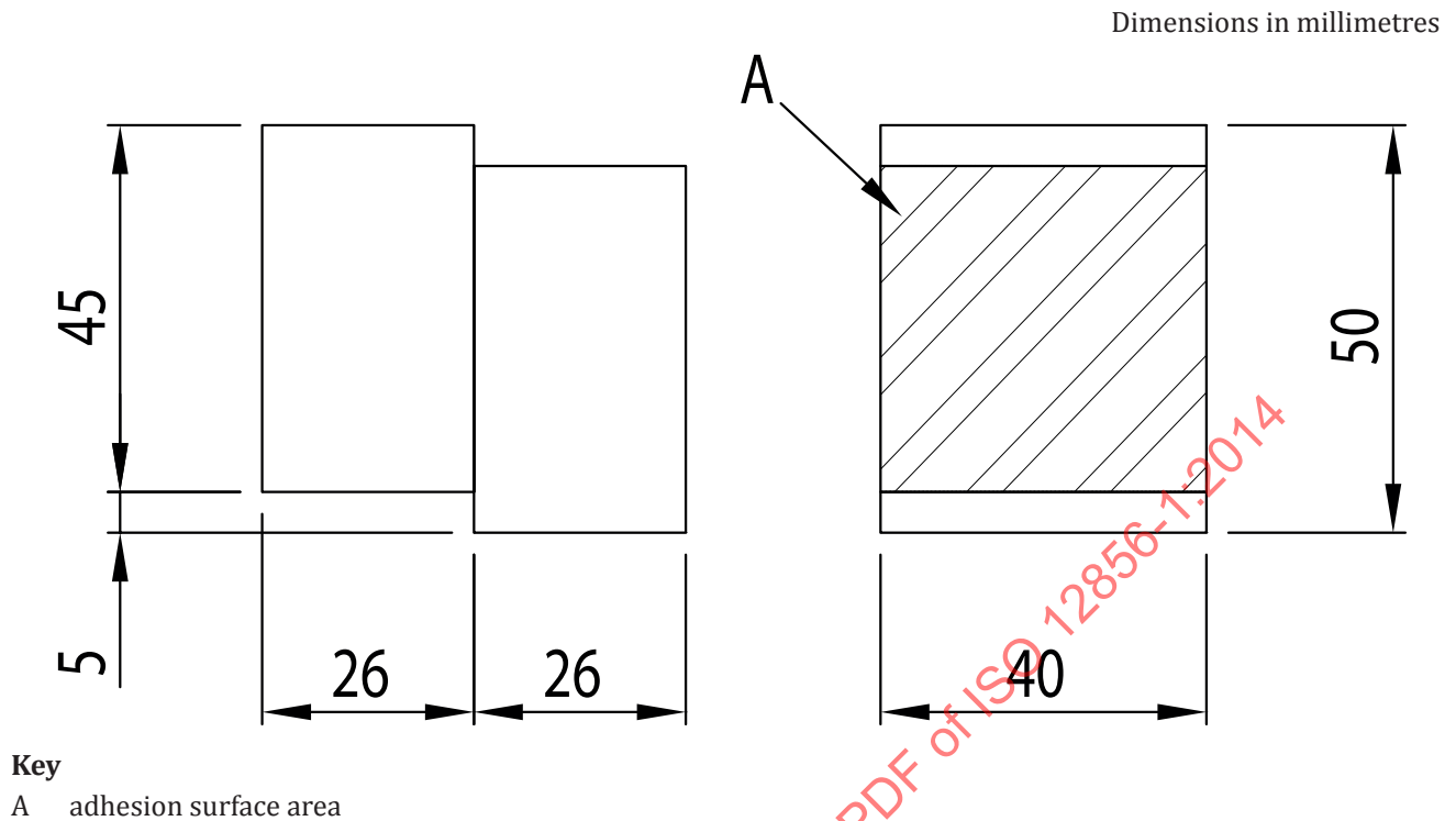
Figure 4 — Test specimen for shear strength test
