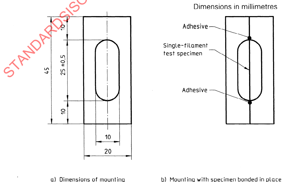
Figure 1 — Mounting for single-filament test specimen
