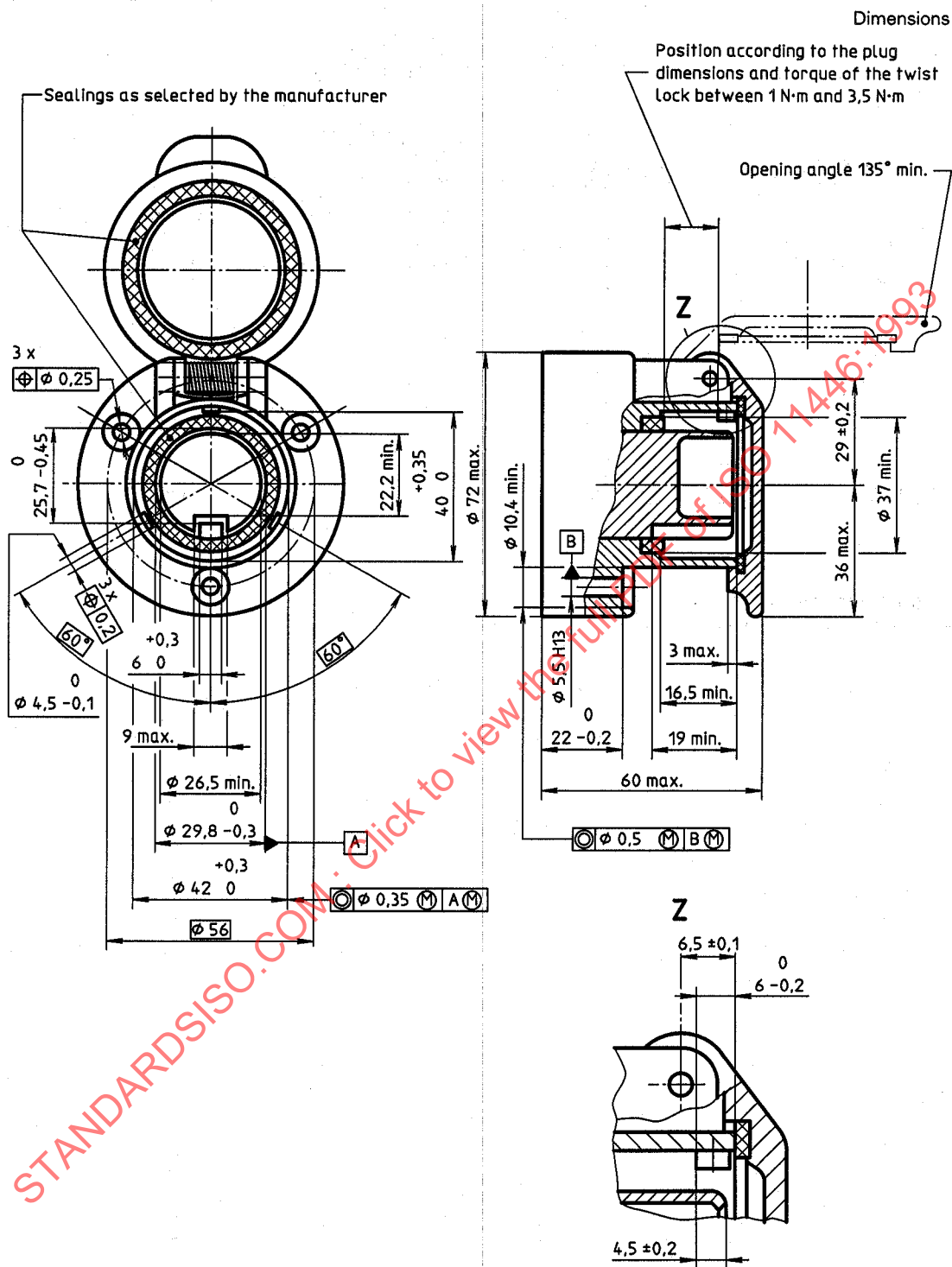
Figure 3 — Park socket
