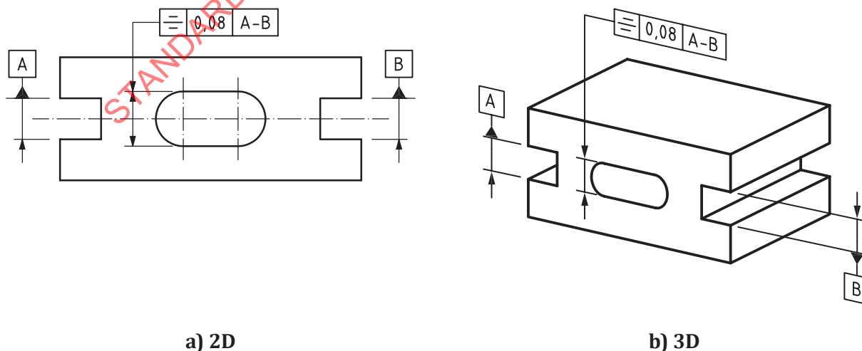
Figure 170 — Symmetry indication
