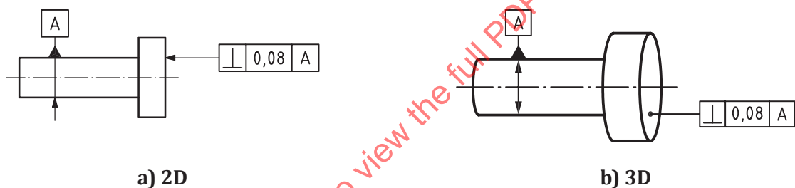
Figure 136 — Perpendicularity indication
