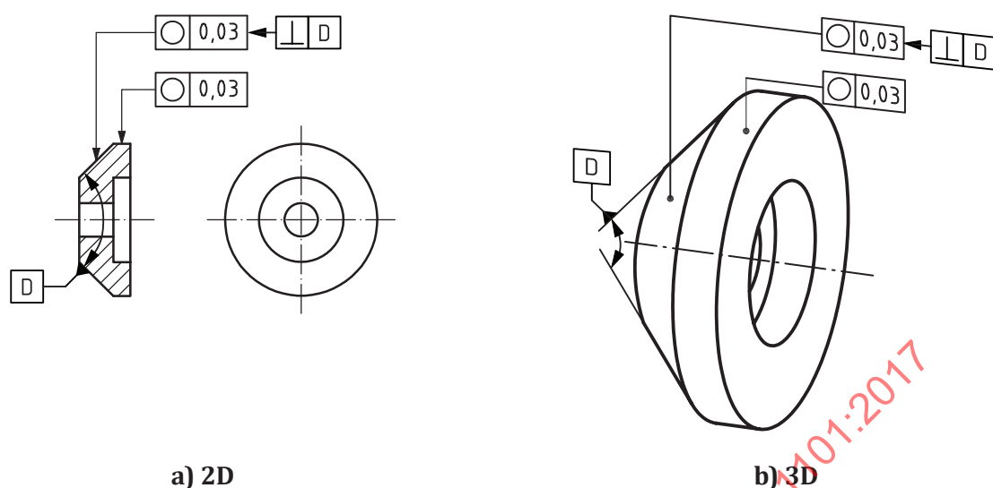
Figure 98 — Roundness indication
