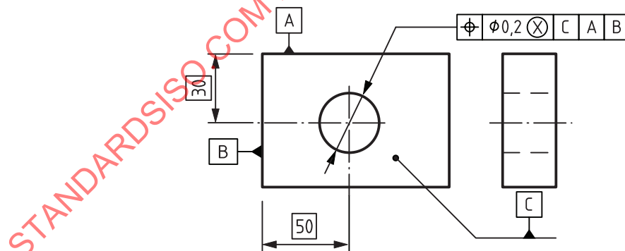
Figure 33 — Maximum inscribed associated tolerated feature — Drawing indication
