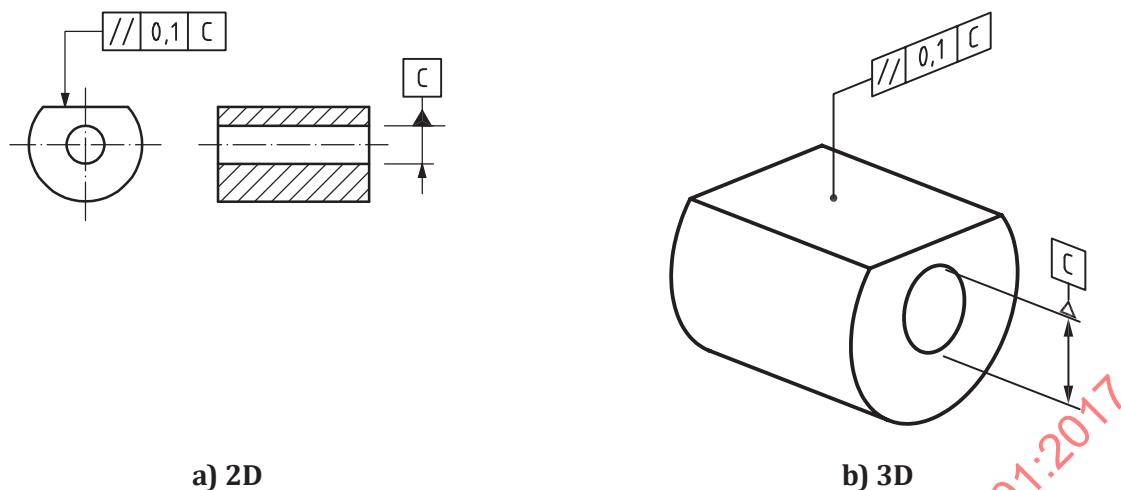
Figure 124 — Parallelism indication
