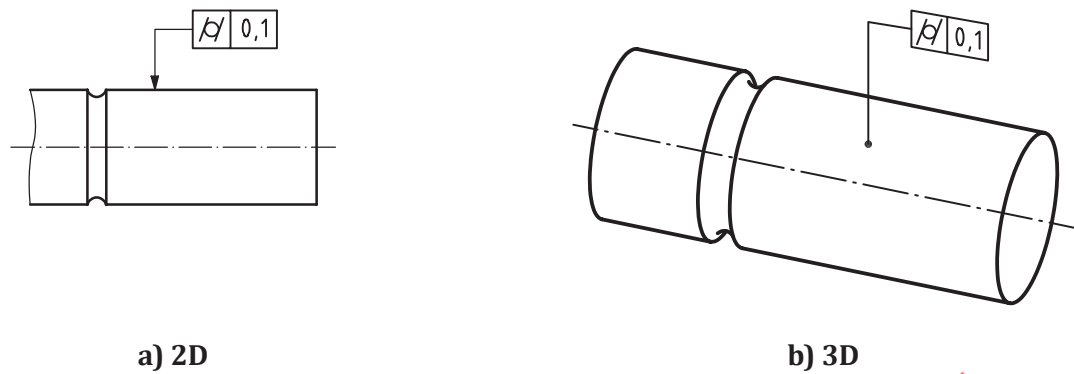
Figure 102 — Cylindricity indication
