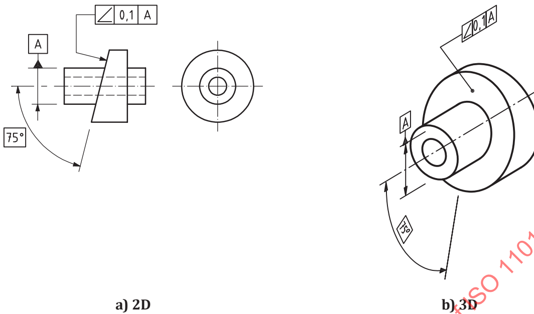
Figure 146 — Angularity indication
