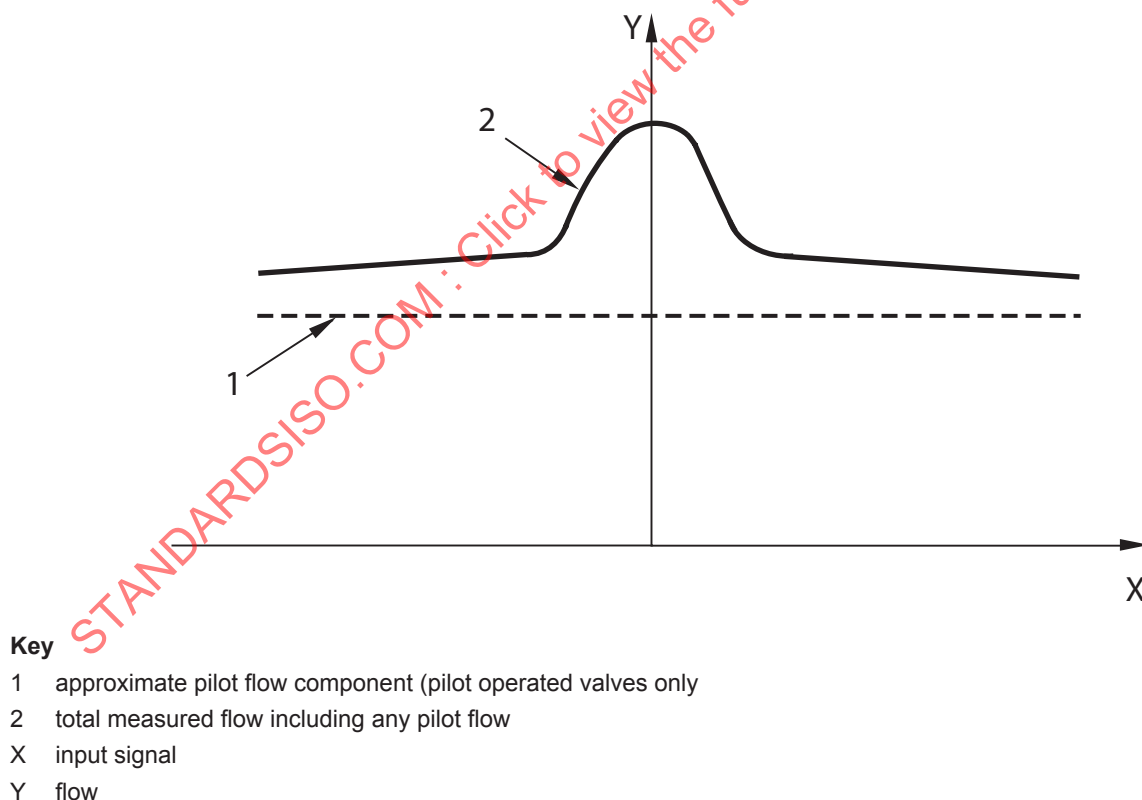
Figure 3 — Internal leakage measurement
