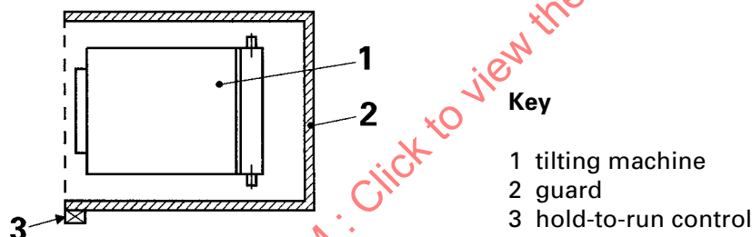
Figure 2 — Safeguarding of tilting machines controlled manually
