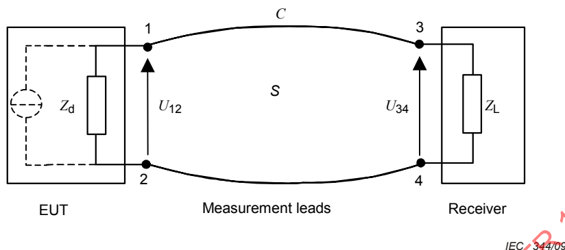
Figure 12 – Basic circuit of a voltage measurement
