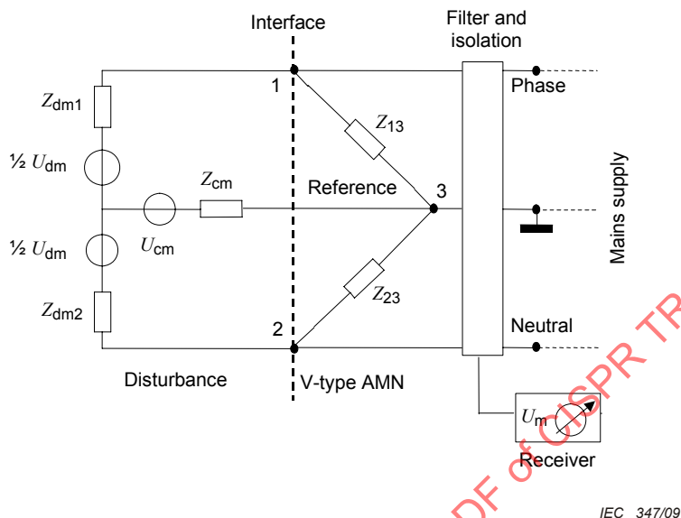
Figure 15 – Basic circuit of the V-AMN voltage measurement ( N = 2 )
