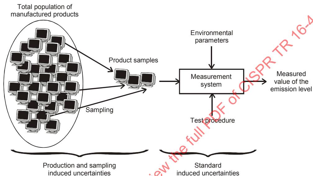
Figure 2 – The process of emission compliance measurements and the associated (categories of) uncertainty sources (see also Table 2)
