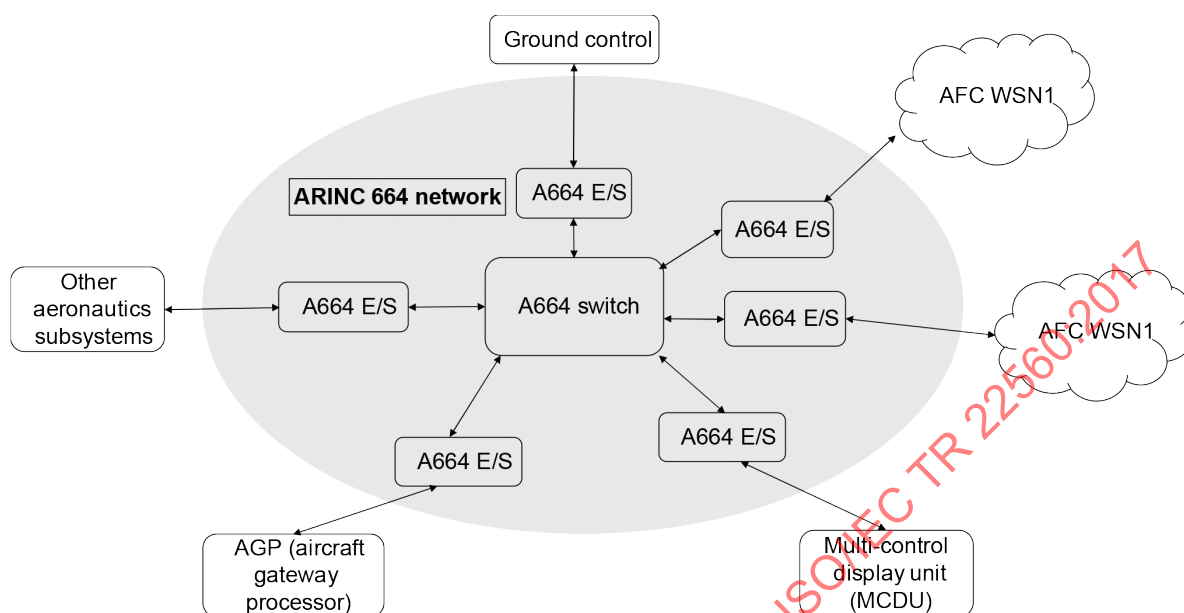
Figure 6 – Interaction with internal avionics networks
