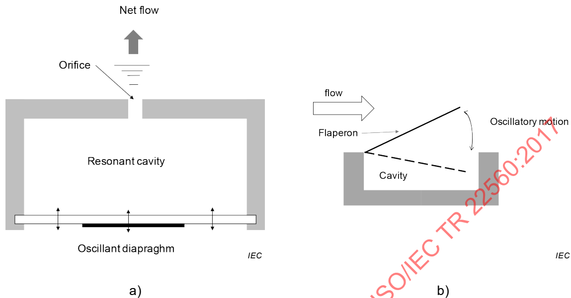
Figure 8 – Flow control actuators: a) SJA; b) flaperon
