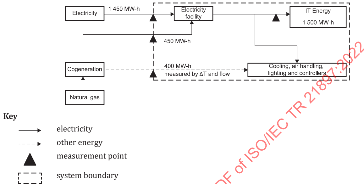
Figure A.5 — Method 1: Measurement of chilled water flow
