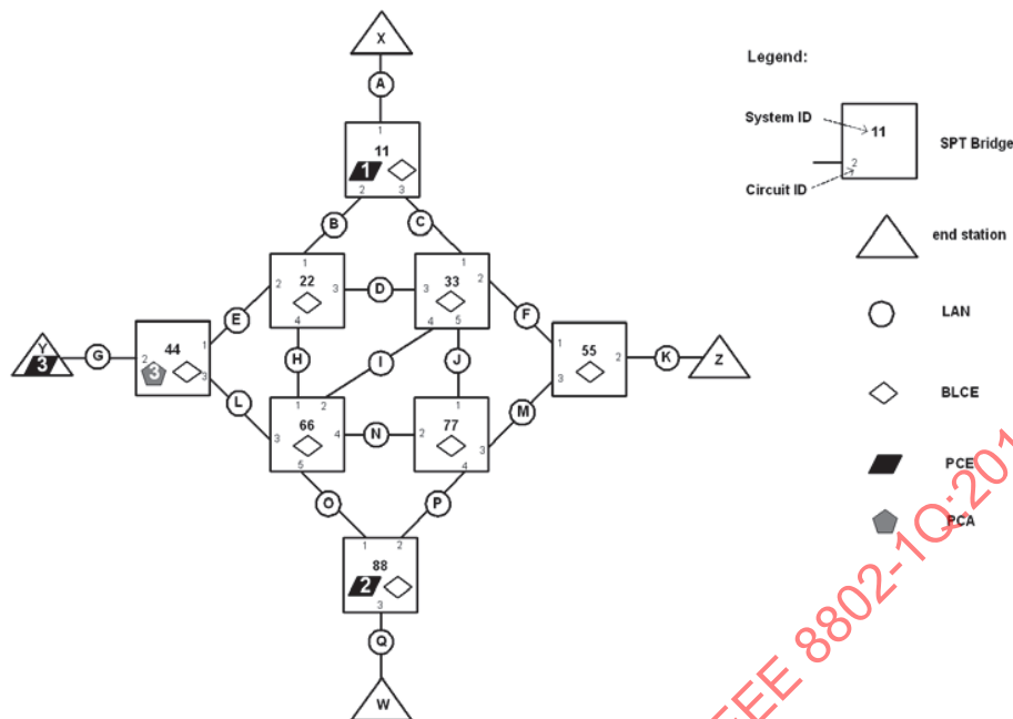
Figure 45-2—An SPT Region controlled by multiple PCEs
