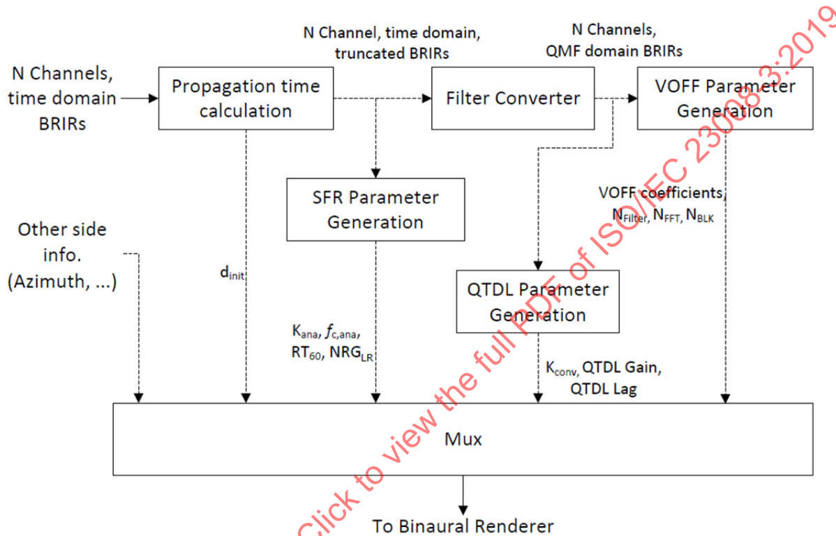
Figure 78 — Details of BRIR parameterization
