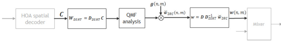
Figure 40 — DRC-1 gain application for HOA in the QMF-domain combined with rendering step
