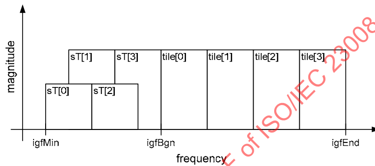
Figure 13 — Computing target tiles, overview
