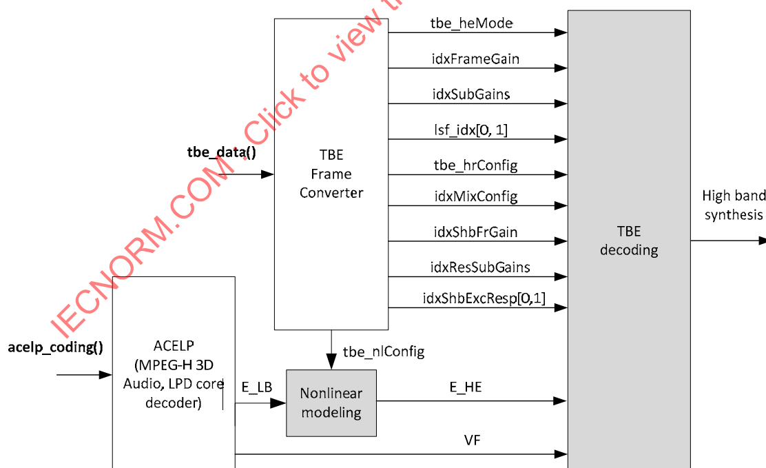
Figure 19 — TBE decoder tools
