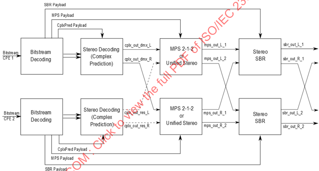
Figure 8 — QCE decoder schematics
