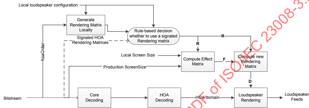
Figure 103 — Screen-related processing for higher order ambisonics
