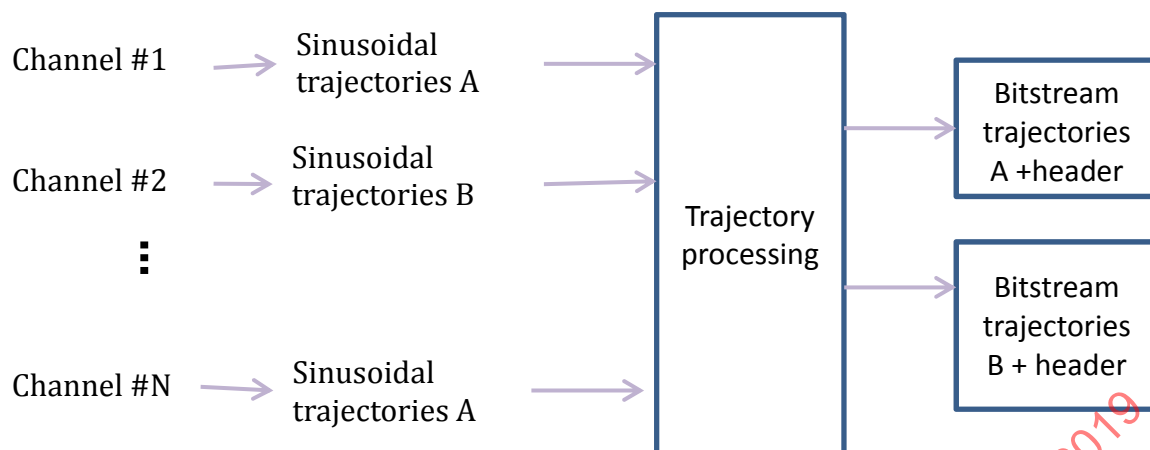
Figure 26 — Sending additional information related to trajectory panning
