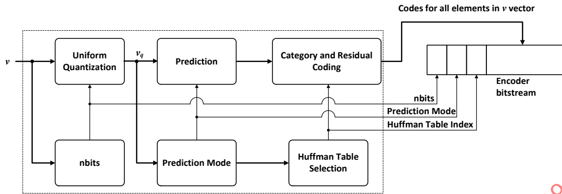
Figure 60 — Coding of V-vector
