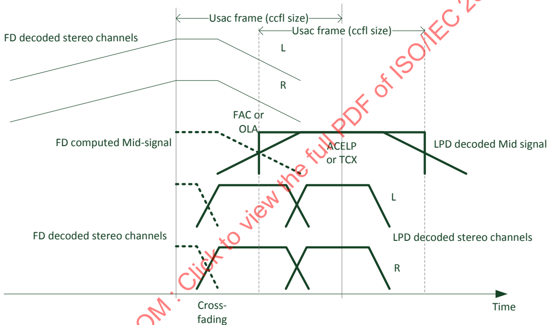
Figure 23 — Schematic representation of the transition from FD to LPD mode with LPD stereo
