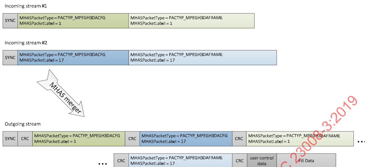
Figure 97 — Example output bitstream from MHAS merger
