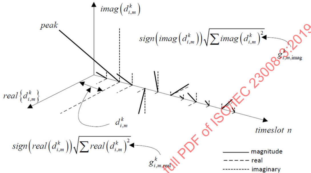
Figure 79 — Geometric descriptions of QTDL parameters
