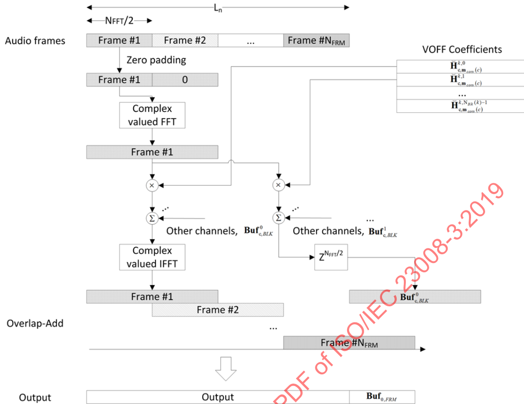
Figure 80 — Outlines of the partitioned fast convolution process
