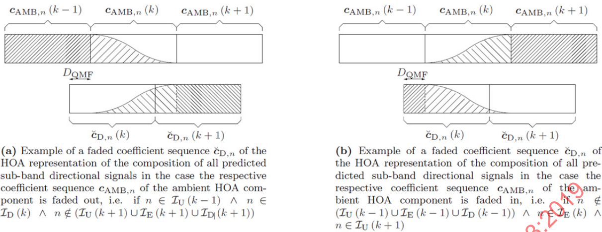
Figure 68 — Illustration of faded coefficient sequences of \check{c}_D(k)
