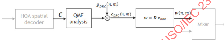
Figure 41 — DRC-1 gain application for HOA in the QMF-domain combined with rendering step for the simple case of a single DRC channel group
