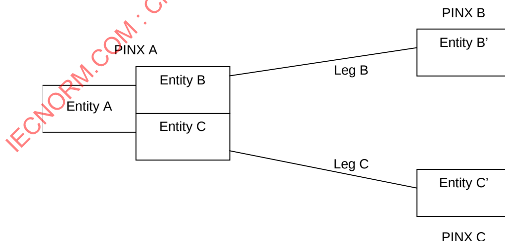
Figure 2 – Call transfer by join model for QSIG
