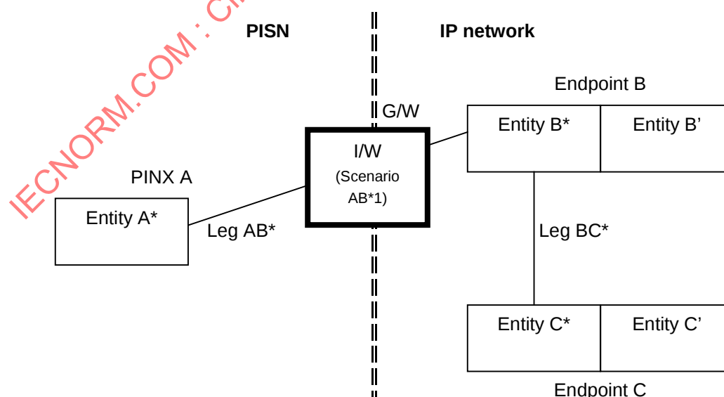
Figure 18 – Interworking – single step call transfer between PINX A and endpoints B and C in the IP network
