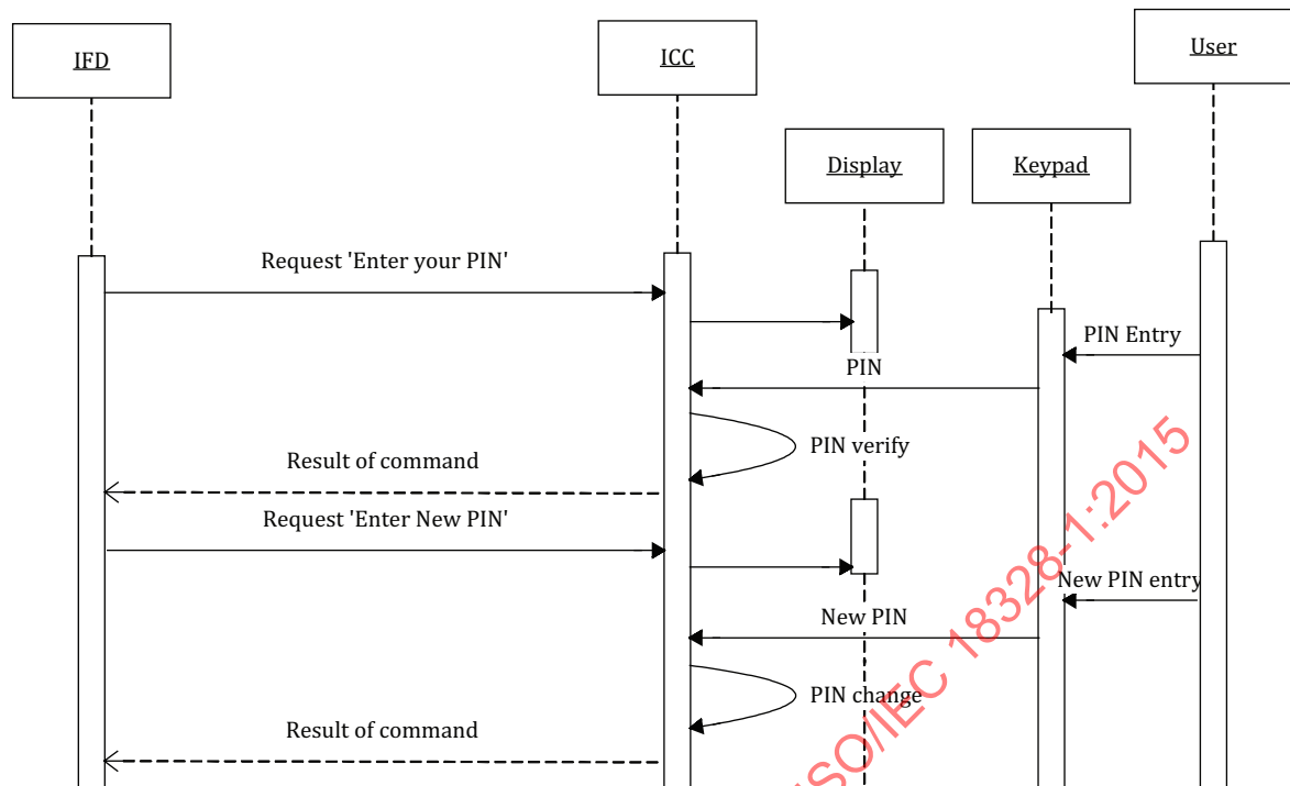
Figure B.1 — Reference data changing with on-card display and keypad on ICC
