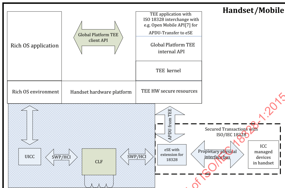
Figure B.3 — ISO/IEC 18328 usage in a handset environment
