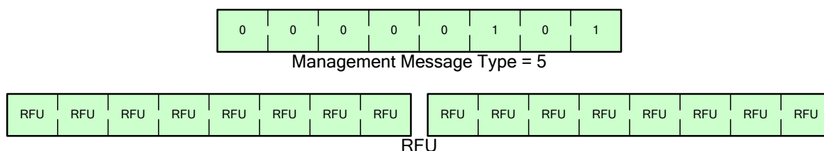
Figure 16 — DAS-RSP message format
