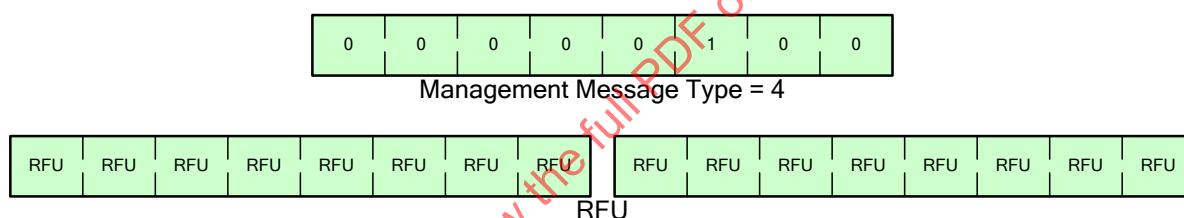
Figure 15 — DAS-REQ message format
