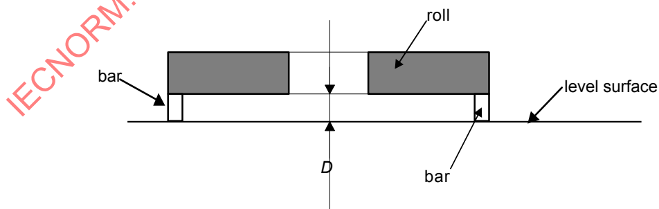
Figure 2 — Tightness of reel winding
