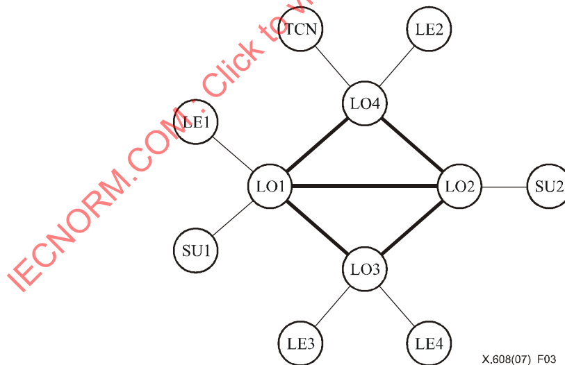
Figure 3 – A two-layer tree for N-plex multicast connection
