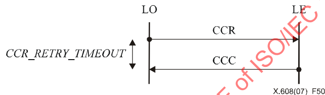
Figure 50 – Control tree change procedures
