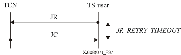
Figure 37 – Late joining procedures
