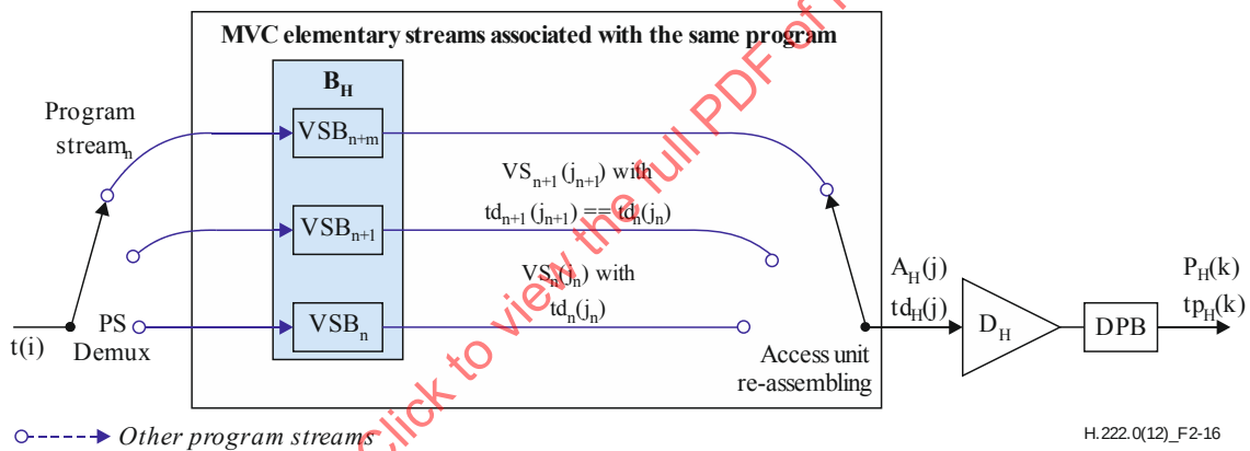
Figure 2-16 – P-STD model extensions for Rec. ITU-T H.222.0 | ISO/IEC 14496-10 Video with MVC video sub-bitstreams
