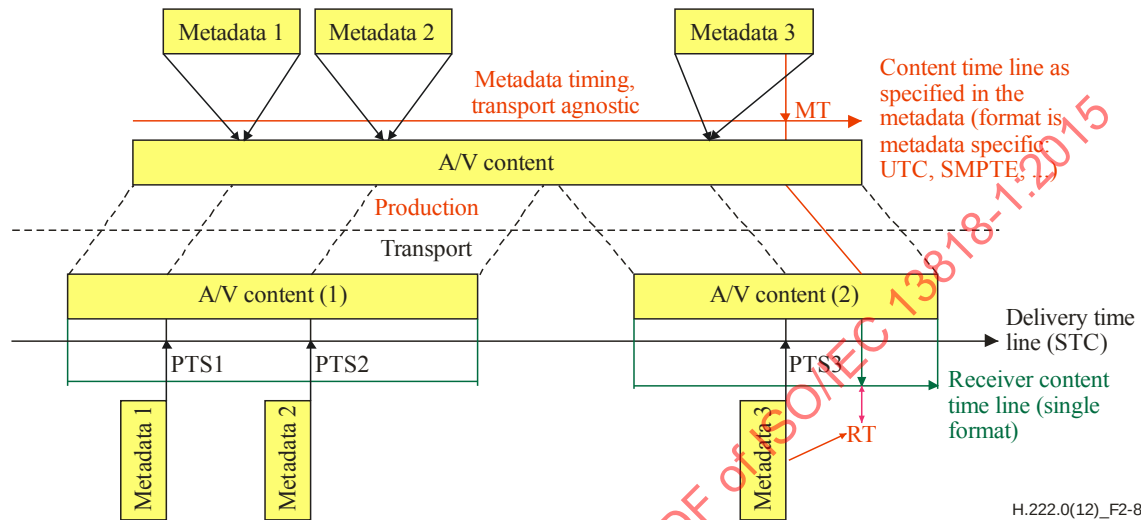
Figure 2-8 – Delivery of metadata in PES packets
