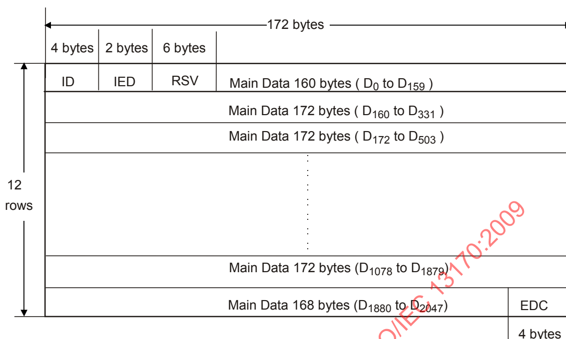
Figure 28 — Data Frame
