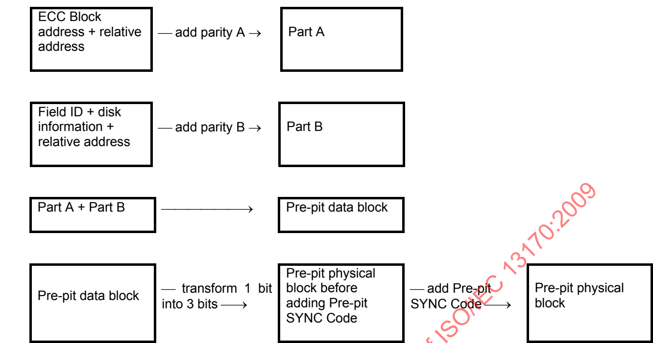
Figure 53 — Processing order to construct a Pre-pit block
