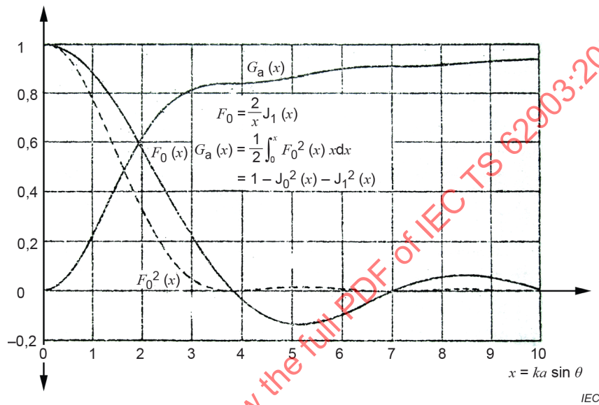
Figure E.2 – Function G_a(ka \sin \theta) , diffraction pattern F_0(ka \sin \theta) and F_0^2(ka \sin \theta) in the geometric focal plane [10]
