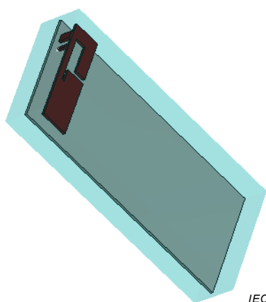
Figure 13 – Generic mobile phone with integrated multiband patch antenna
