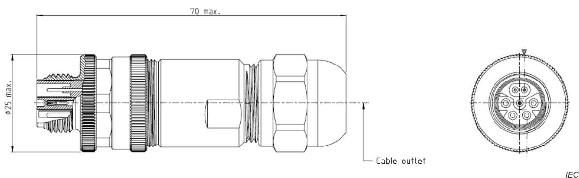
Figure 4 – Styles 6P-P12C and 6P-M12C overall dimensions
