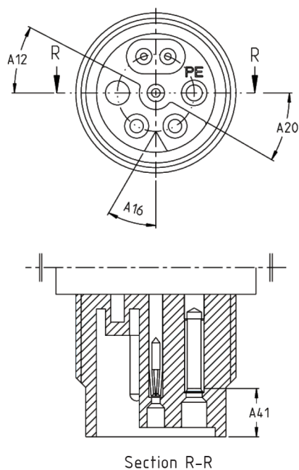
Figure 7 – Dimensions of PE pin for the codings Type I to V and styles with male contacts (at the example of coding Type IV)
