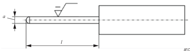
Figure 10 – Gauge dimensions
