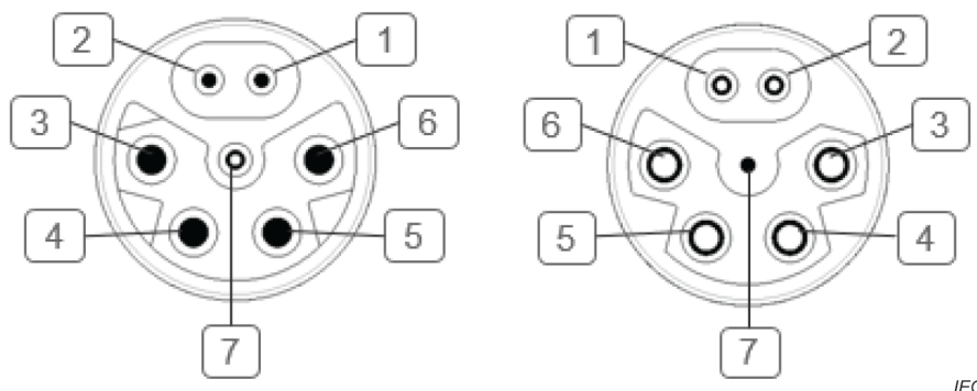
Figure 11 – Pin assignments, front views, Types I and II
