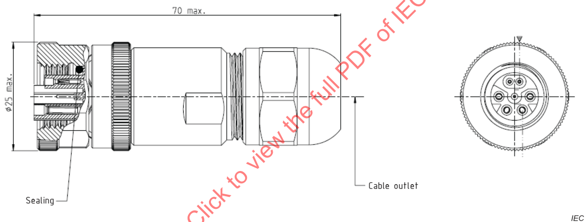
Figure 5 – Styles 6P-P12CI and 6P-M12CI overall dimensions
