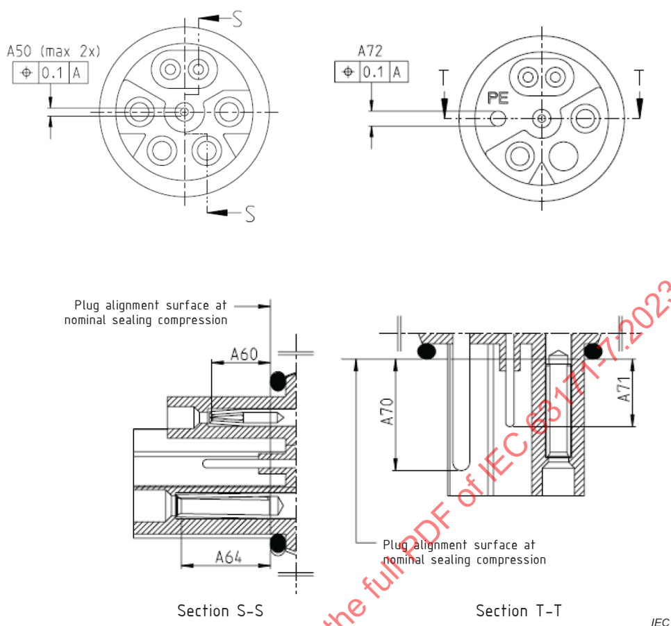
Figure 9 – Mating dimensions for the styles with female contacts (at the example of codings Type I and Type IV)
