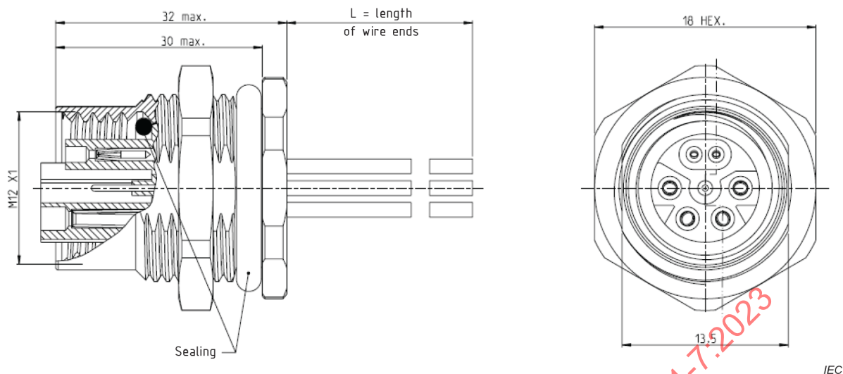
Figure 2 – Styles 6J-P12C, 6J-M12C, 6J-C12C overall dimensions
