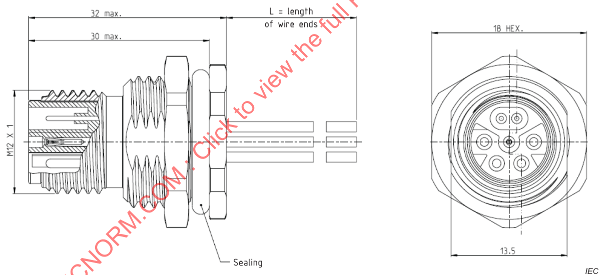
Figure 3 – Styles 6J-P12CI, 6J-M12CI and 6J-C12CI overall dimensions
