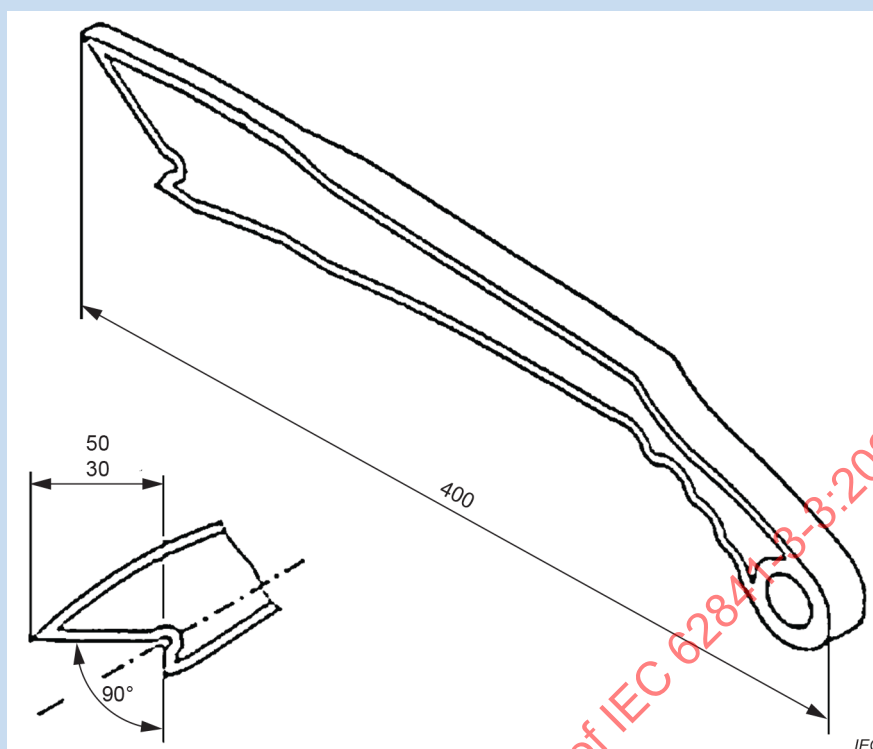
Figure 111 – Example of a push stick
