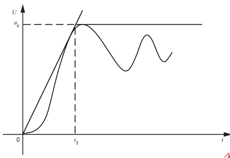
Figure 4 – Example of a two parameters envelope for a TRV
