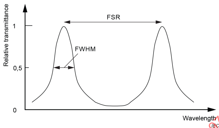
Figure A.2 – Transmission characteristic of an etalon
