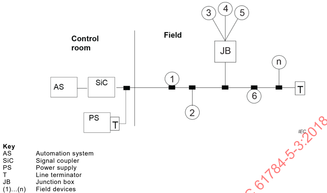
Figure B.8 – Combination of the tree topology and the bus topology
