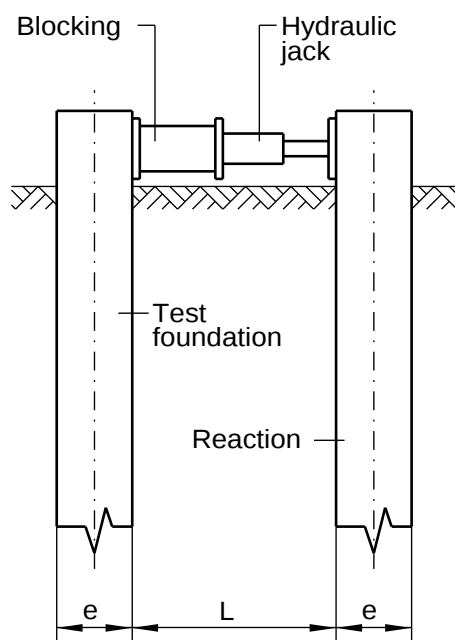
Figure 6a – Reaction foundation, pushing apart
