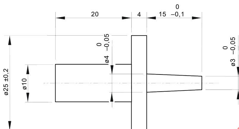
Figure 3 – Test pin (see IEC 61032, test probe 13)
