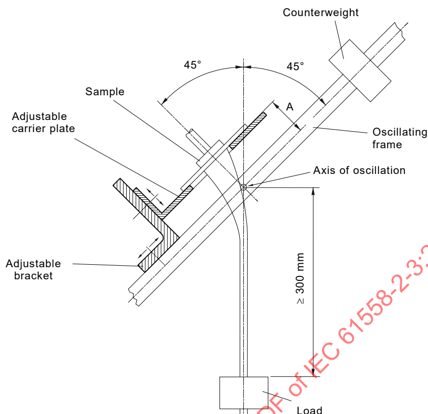
Figure 11 – Flexing test apparatus
