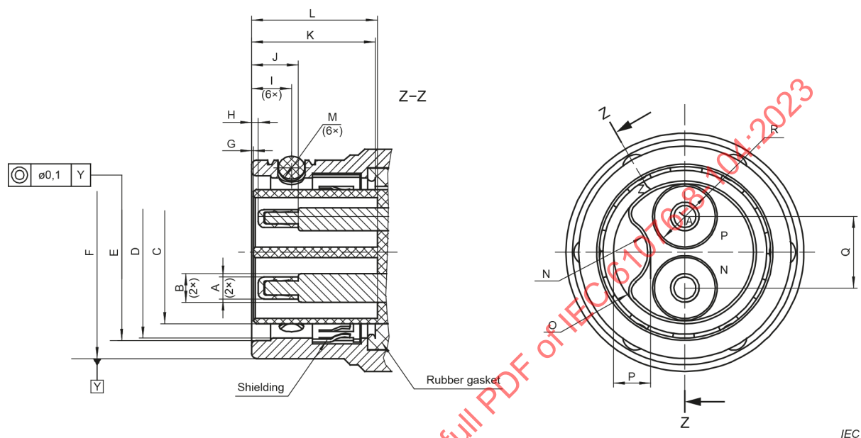
Figure 4 – Fixed connector
