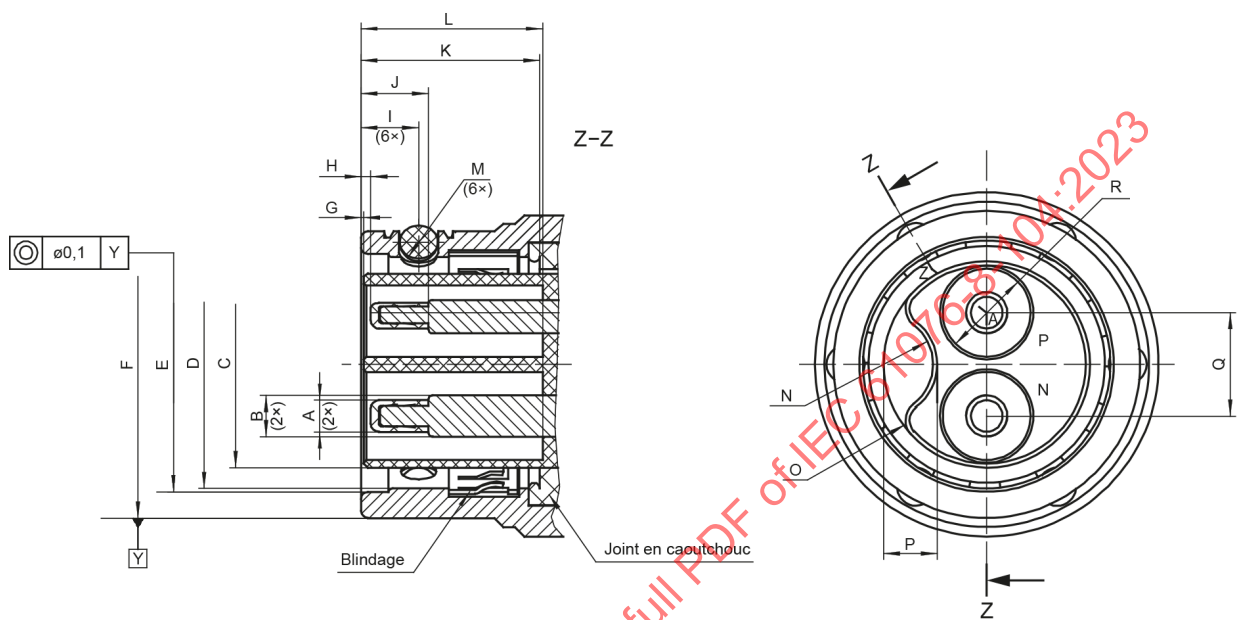
Figure 4 – Embase
