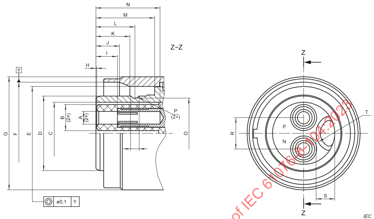
Figure 3 – Free connector
