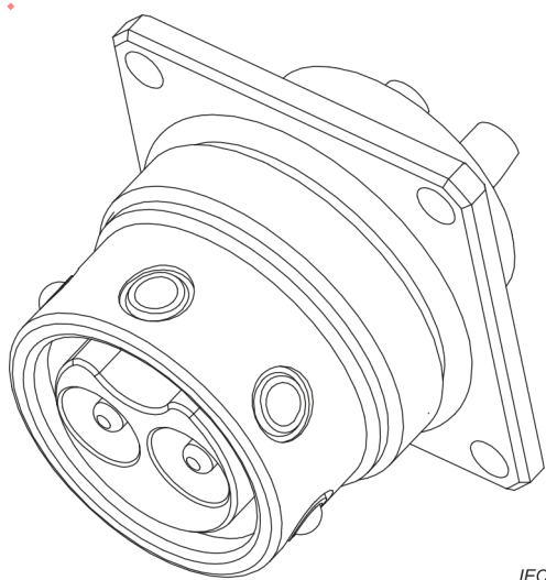
Figure 2 – Embase
