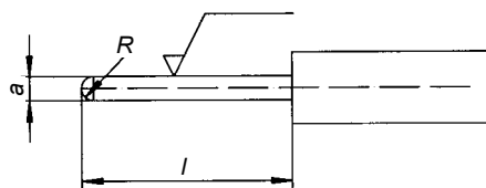
Figure 22 – Gauge dimensions
