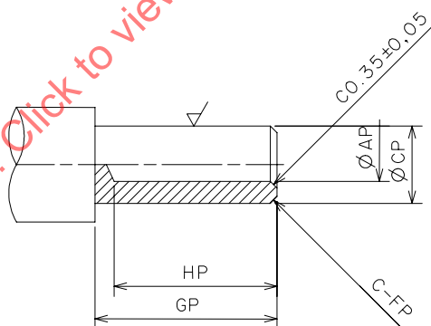
Figure 4a – Plug gauge style A
