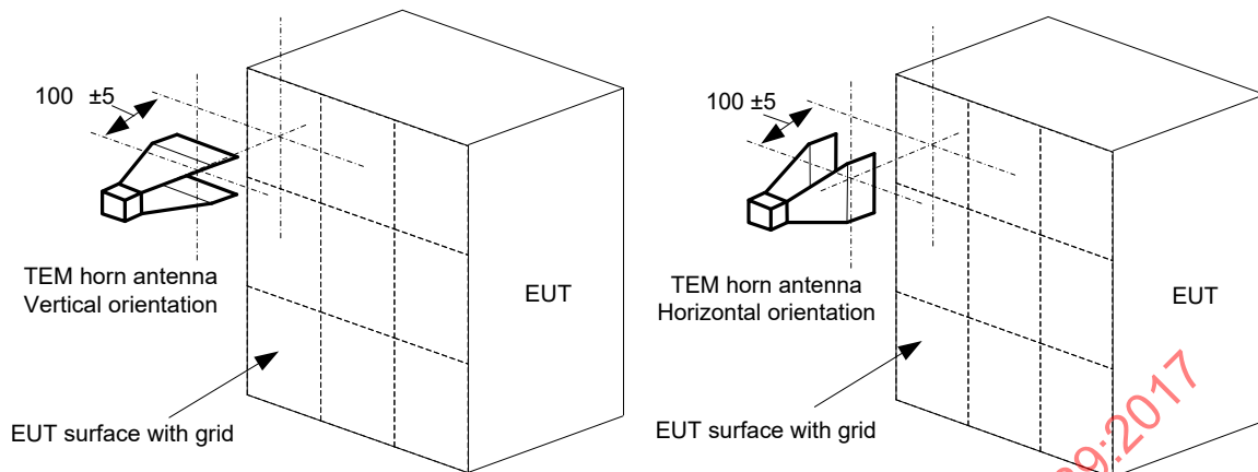
Figure 12 – Example of TEM horn antenna orientations
