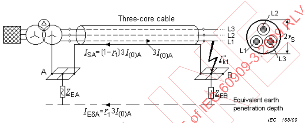
a) Feeding from station A only and line-to-earth short circuit in station B
