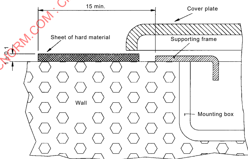
Figure 13 – Arrangement for test on cover-plates
