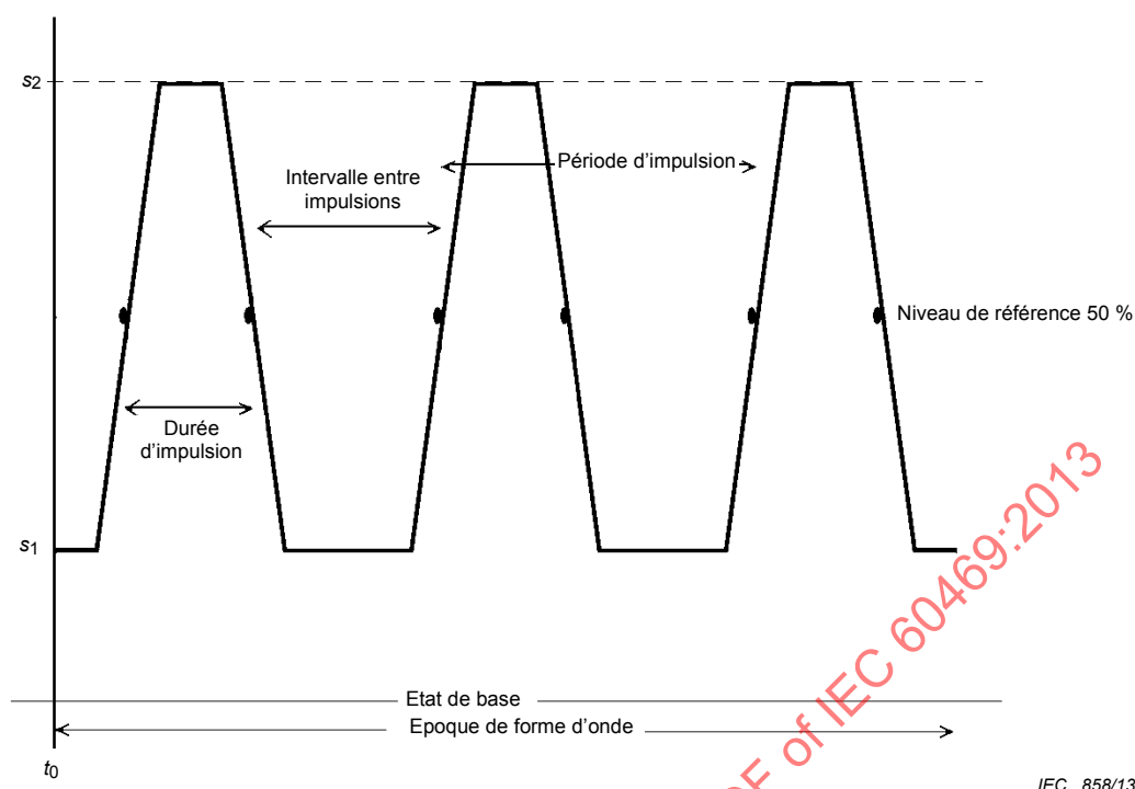
Figure 7 – Train d'impulsions
