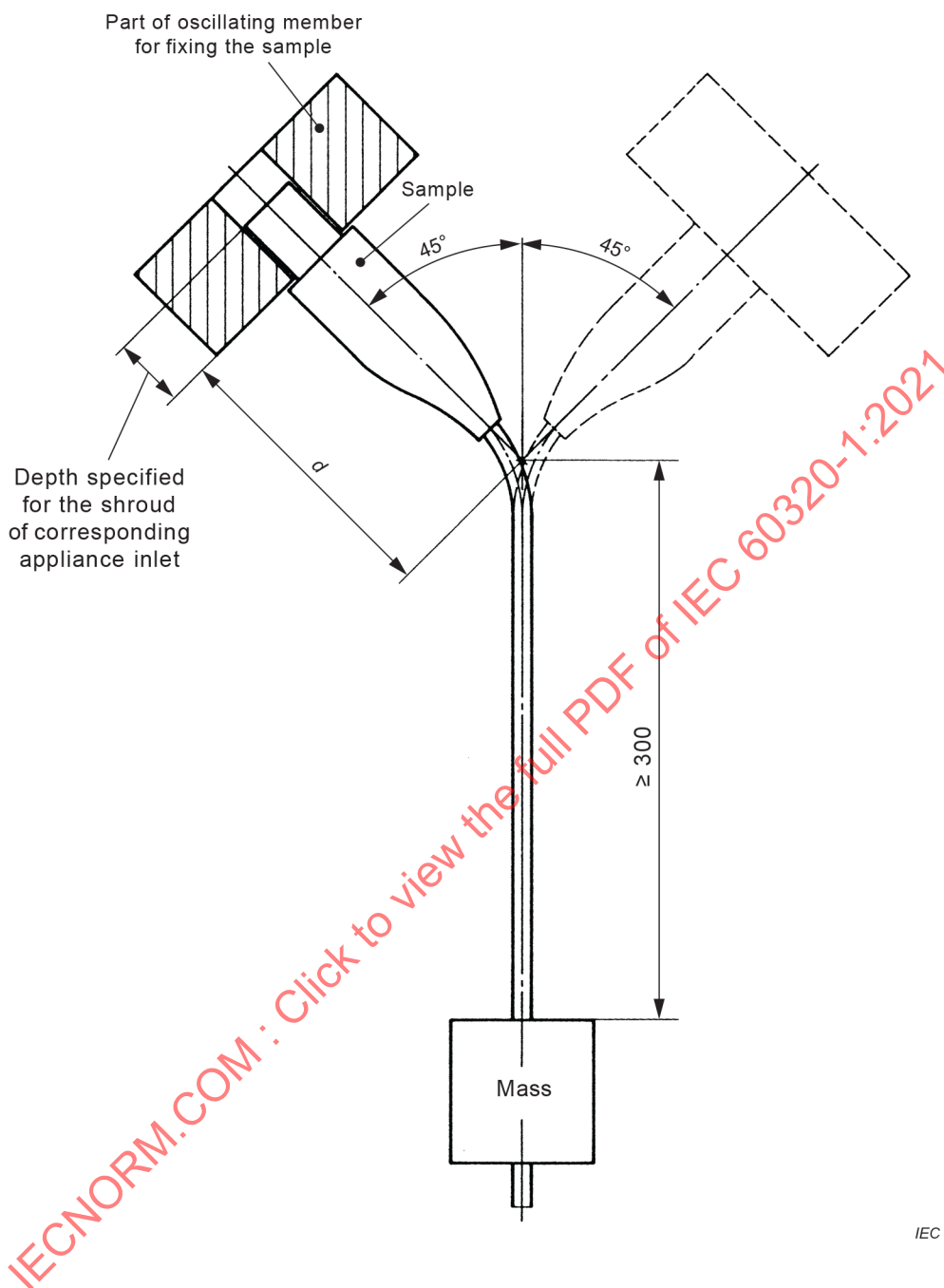
Figure 8 – Apparatus for the flexing test
